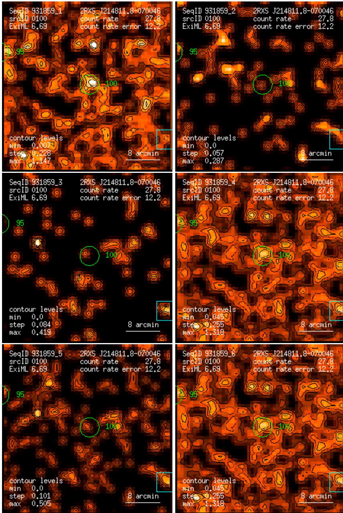
Figure 100: RASS 931859: detection 0100: band rate images, Gaussian filter: (1) PSPC channels 11 – 41, (2) 52 – 90, (3) 91 – 201, (4) 11 – 235, (5) 52 – 201, (6) 11 – 201. Broad band rates in counts/ks. Band rate contour levels in counts/ks/arcmin 2 .
