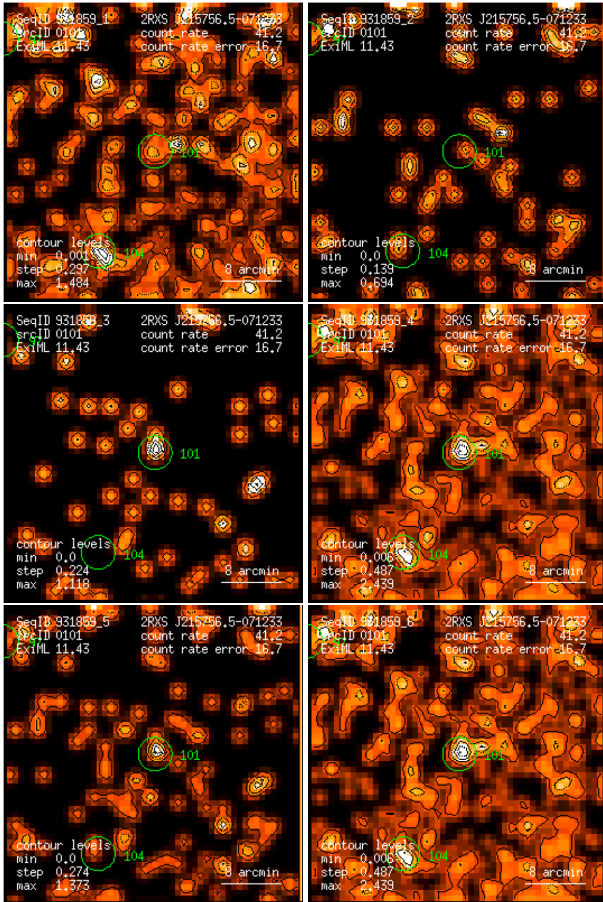
Figure 101: RASS 931859: detection 0101: band rate images, Gaussian filter: (1) PSPC channels 11 – 41, (2) 52 – 90, (3) 91 – 201, (4) 11 – 235, (5) 52 – 201, (6) 11 – 201. Broad band rates in counts/ks. Band rate contour levels in counts/ks/arcmin 2 .
