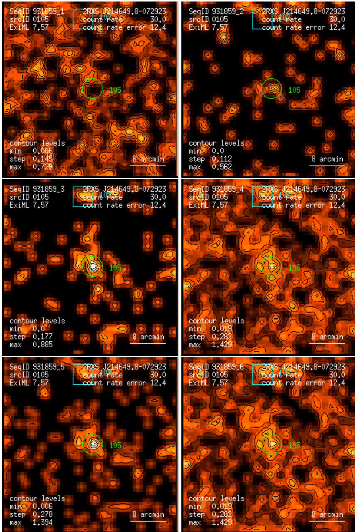
Figure 105: RASS 931859: detection 0105: band rate images, Gaussian filter: (1) PSPC channels 11 – 41, (2) 52 – 90, (3) 91 – 201, (4) 11 – 235, (5) 52 – 201, (6) 11 – 201. Broad band rates in counts/ks. Band rate contour levels in counts/ks/arcmin 2 .
