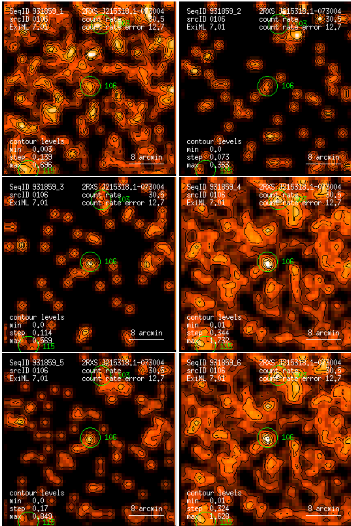
Figure 106: RASS 931859: detection 0106: band rate images, Gaussian filter: (1) PSPC channels 11 – 41, (2) 52 – 90, (3) 91 – 201, (4) 11 – 235, (5) 52 – 201, (6) 11 – 201. Broad band rates in counts/ks. Band rate contour levels in counts/ks/arcmin 2 .
