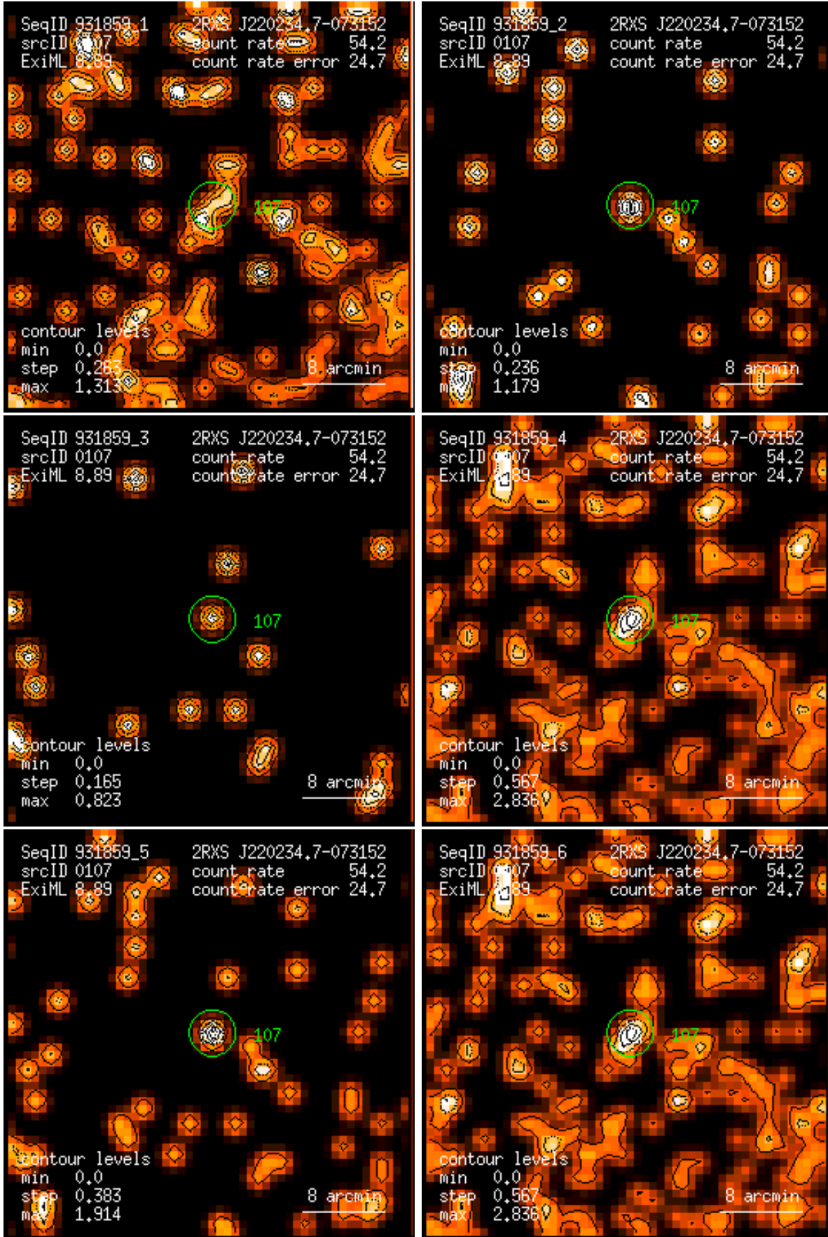
Figure 107: RASS 931859: detection 0107: band rate images, Gaussian filter: (1) PSPC channels 11 – 41, (2) 52 – 90, (3) 91 – 201, (4) 11 – 235, (5) 52 – 201, (6) 11 – 201. Broad band rates in counts/ks. Band rate contour levels in counts/ks/arcmin 2 .
