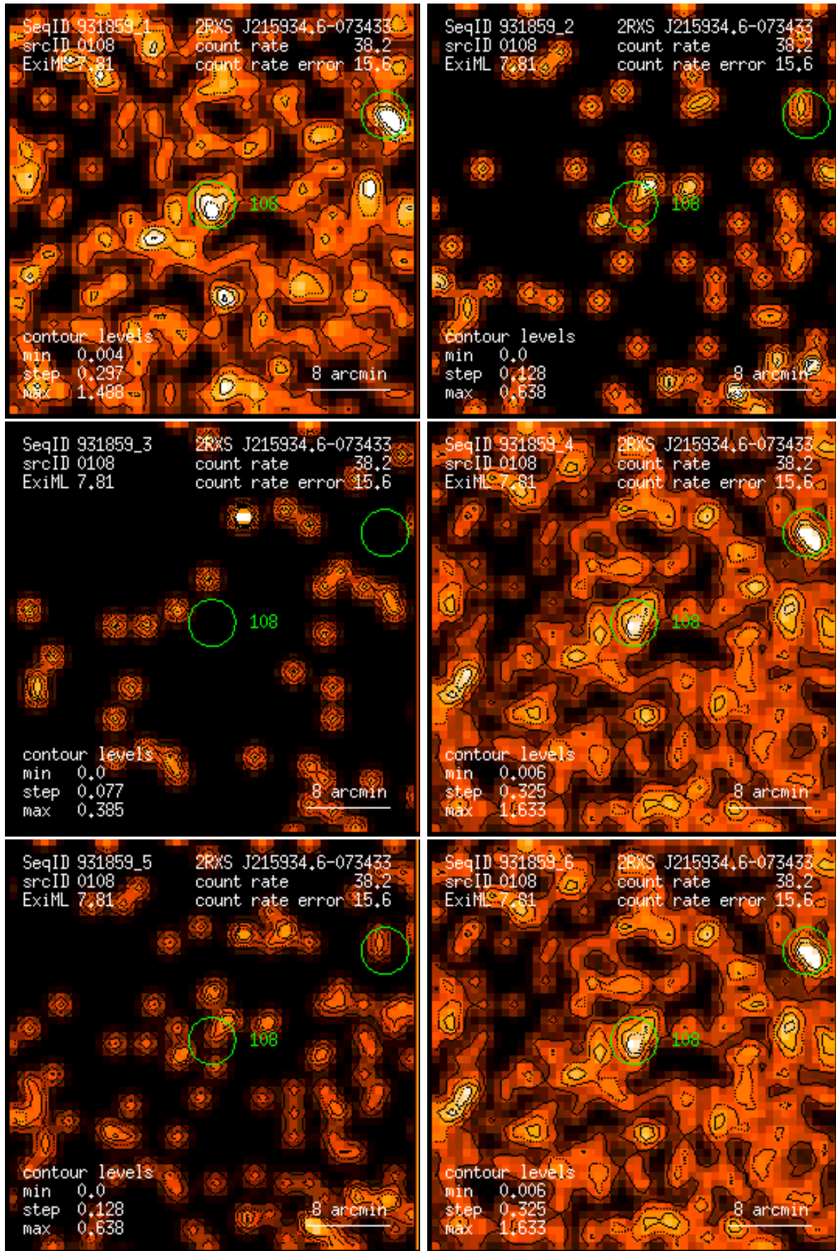
Figure 108: RASS 931859: detection 0108: band rate images, Gaussian filter: (1) PSPC channels 11 – 41, (2) 52 – 90, (3) 91 – 201, (4) 11 – 235, (5) 52 – 201, (6) 11 – 201. Broad band rates in counts/ks. Band rate contour levels in counts/ks/arcmin 2 .
