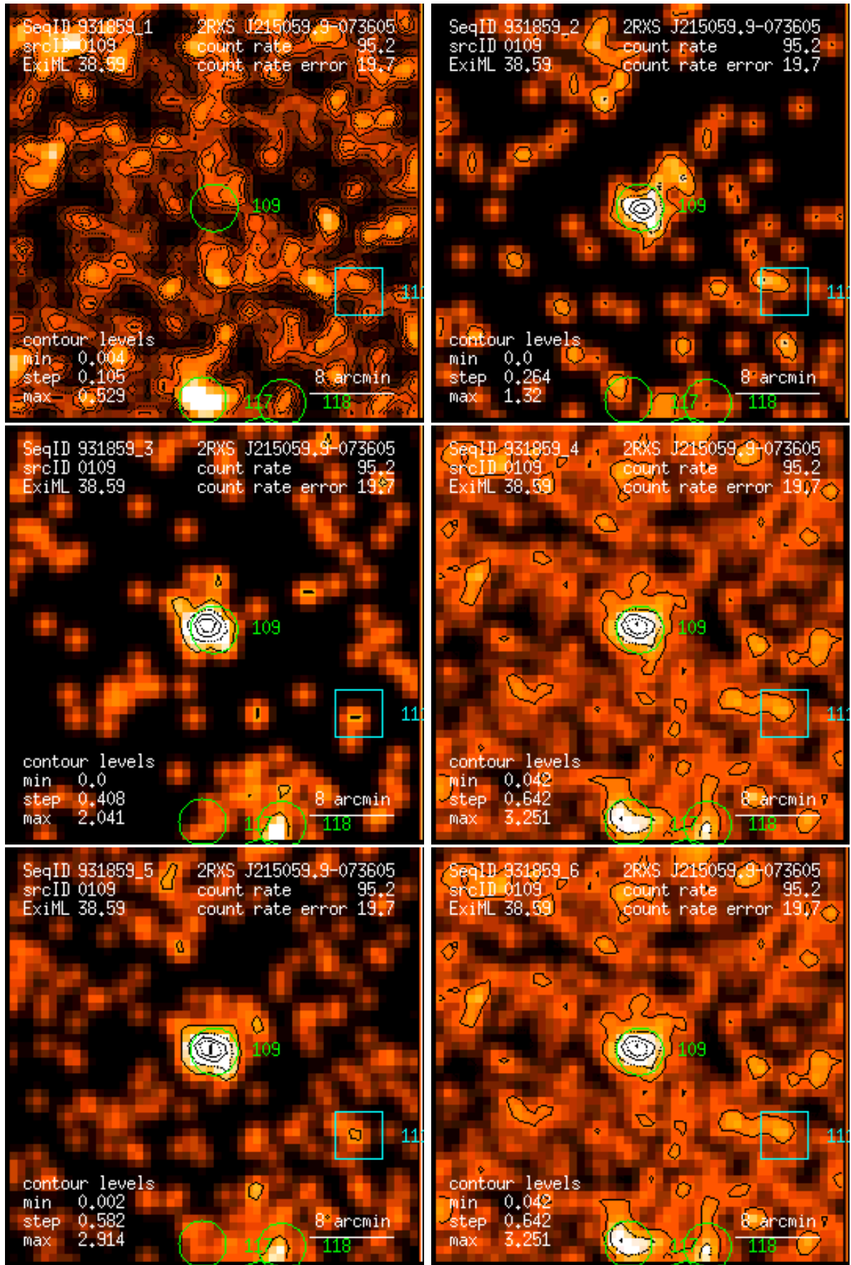
Figure 109: RASS 931859: detection 0109: band rate images, Gaussian filter: (1) PSPC channels 11 – 41, (2) 52 – 90, (3) 91 – 201, (4) 11 – 235, (5) 52 – 201, (6) 11 – 201. Broad band rates in counts/ks. Band rate contour levels in counts/ks/arcmin 2 .
