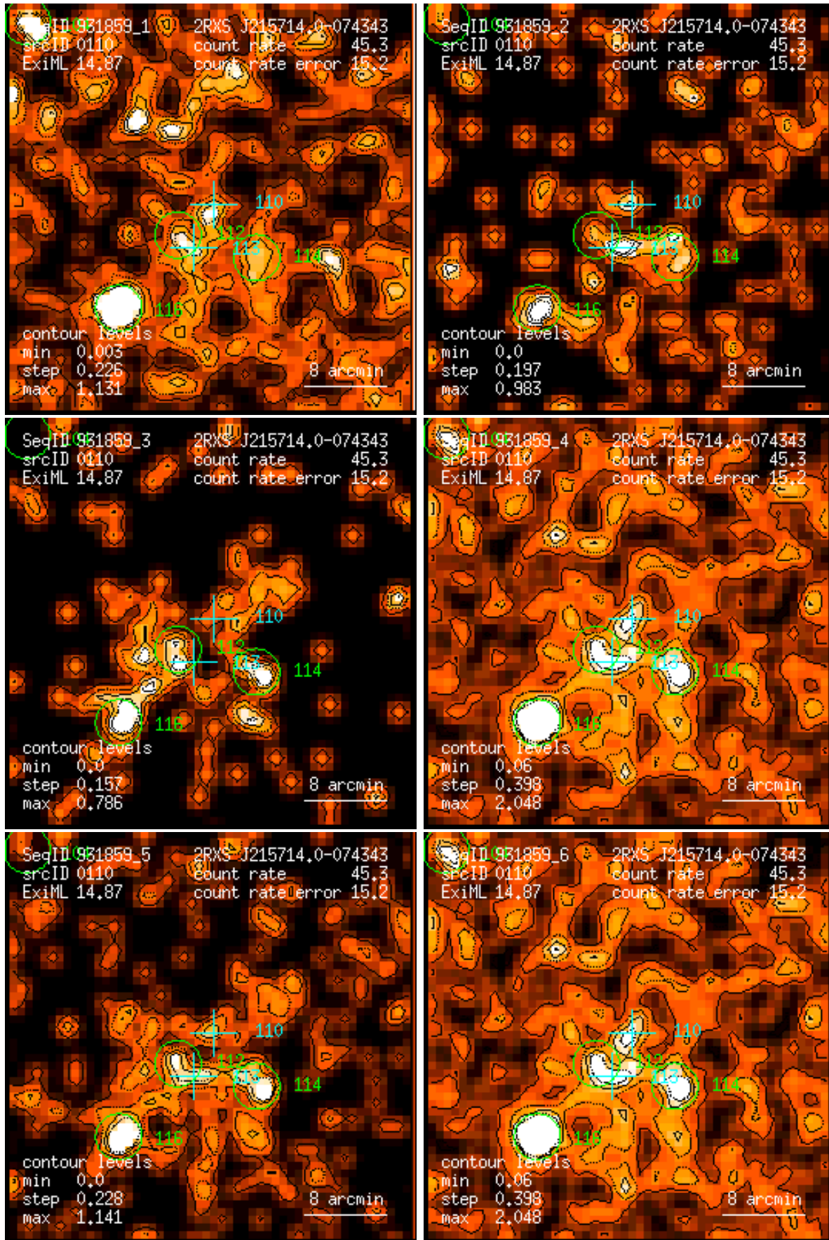
Figure 110: RASS 931859: detection 0110: band rate images, Gaussian filter: (1) PSPC channels 11 – 41, (2) 52 – 90, (3) 91 – 201, (4) 11 – 235, (5) 52 – 201, (6) 11 – 201. Broad band rates in counts/ks. Band rate contour levels in counts/ks/arcmin 2 .
