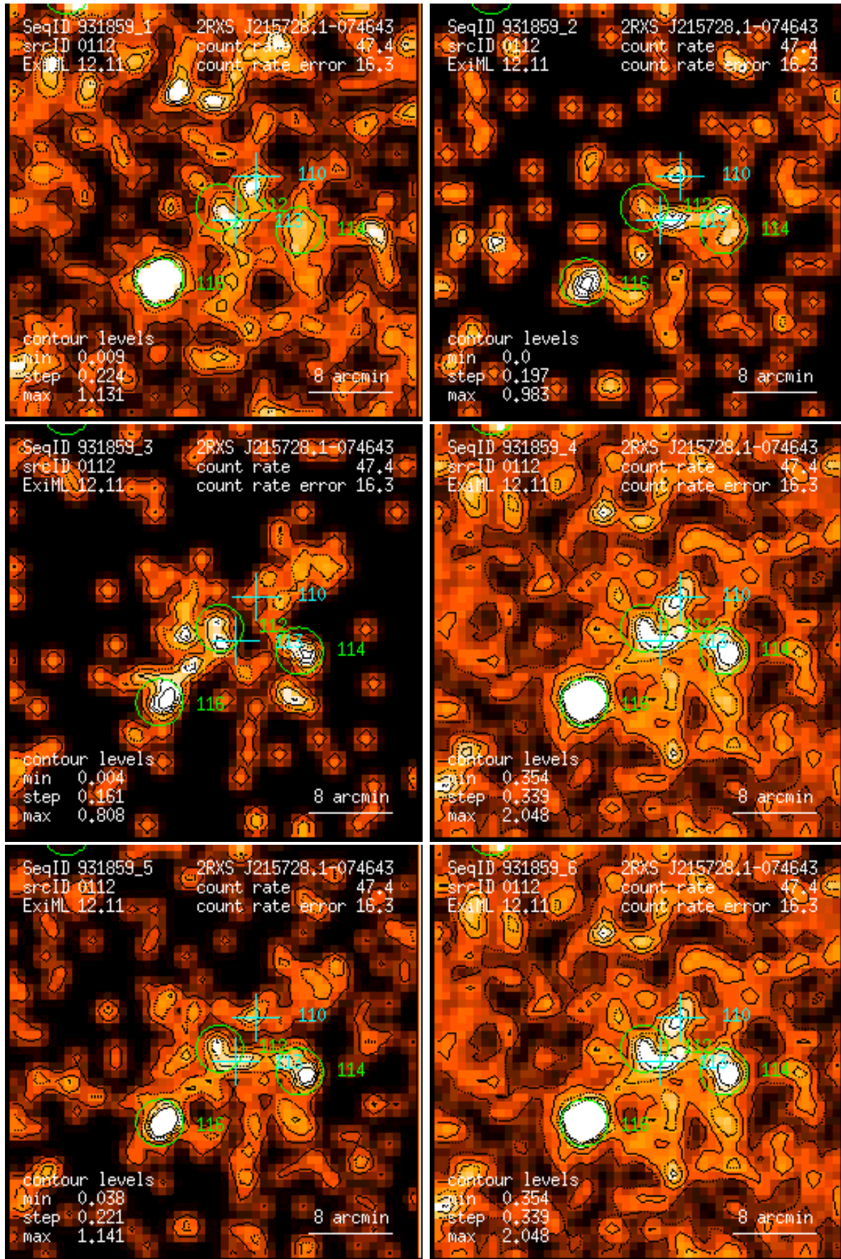
Figure 112: RASS 931859: detection 0112: band rate images, Gaussian filter: (1) PSPC channels 11 – 41, (2) 52 – 90, (3) 91 – 201, (4) 11 – 235, (5) 52 – 201, (6) 11 – 201. Broad band rates in counts/ks. Band rate contour levels in counts/ks/arcmin 2 .
