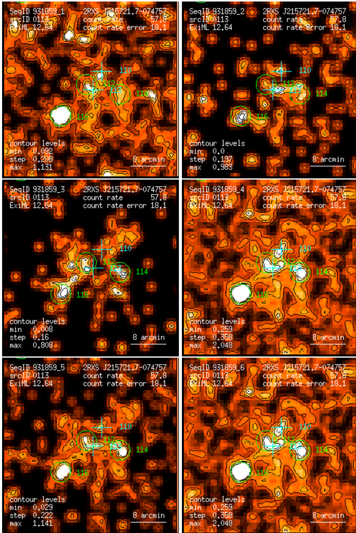
Figure 113: RASS 931859: detection 0113: band rate images, Gaussian filter: (1) PSPC channels 11 – 41, (2) 52 – 90, (3) 91 – 201, (4) 11 – 235, (5) 52 – 201, (6) 11 – 201. Broad band rates in counts/ks. Band rate contour levels in counts/ks/arcmin 2 .
