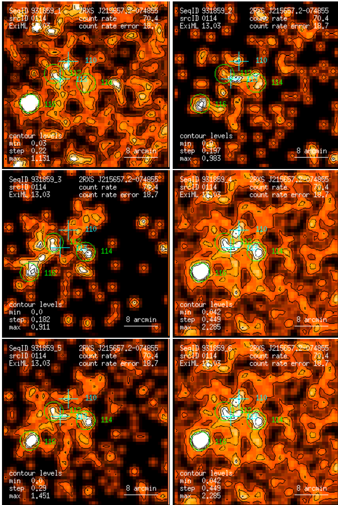
Figure 114: RASS 931859: detection 0114: band rate images, Gaussian filter: (1) PSPC channels 11 – 41, (2) 52 – 90, (3) 91 – 201, (4) 11 – 235, (5) 52 – 201, (6) 11 – 201. Broad band rates in counts/ks. Band rate contour levels in counts/ks/arcmin 2 .
