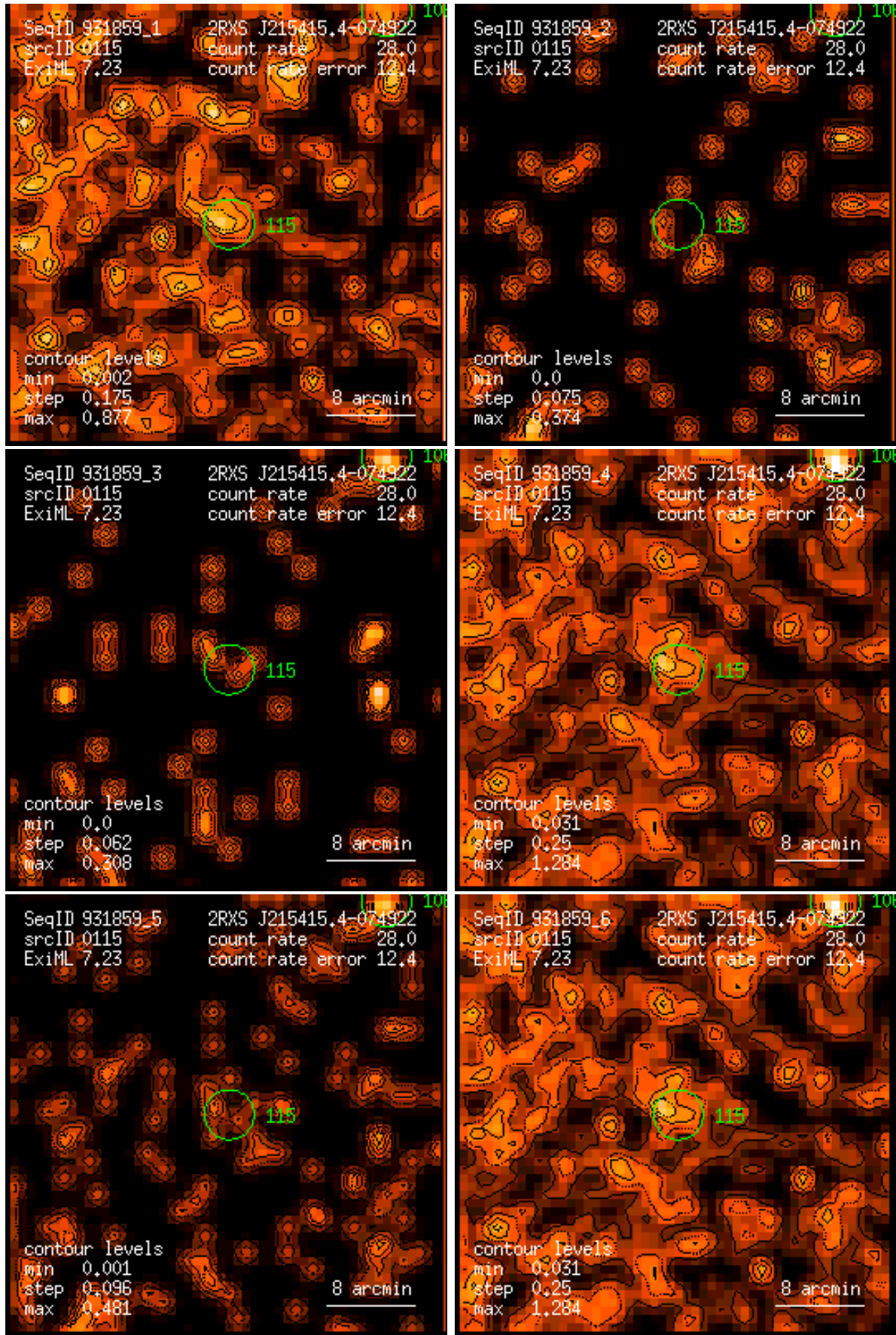
Figure 115: RASS 931859: detection 0115: band rate images, Gaussian filter: (1) PSPC channels 11 – 41, (2) 52 – 90, (3) 91 – 201, (4) 11 – 235, (5) 52 – 201, (6) 11 – 201. Broad band rates in counts/ks. Band rate contour levels in counts/ks/arcmin 2 .
