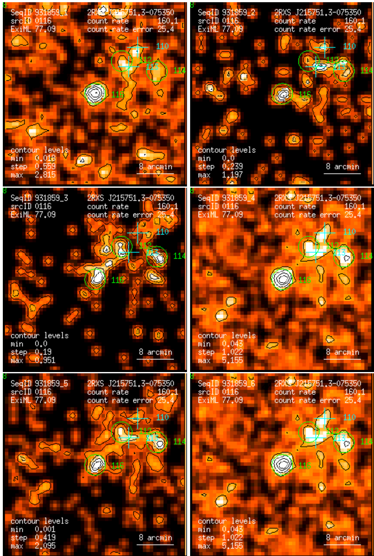
Figure 116: RASS 931859: detection 0116: band rate images, Gaussian filter: (1) PSPC channels 11 – 41, (2) 52 – 90, (3) 91 – 201, (4) 11 – 235, (5) 52 – 201, (6) 11 – 201. Broad band rates in counts/ks. Band rate contour levels in counts/ks/arcmin 2 .
