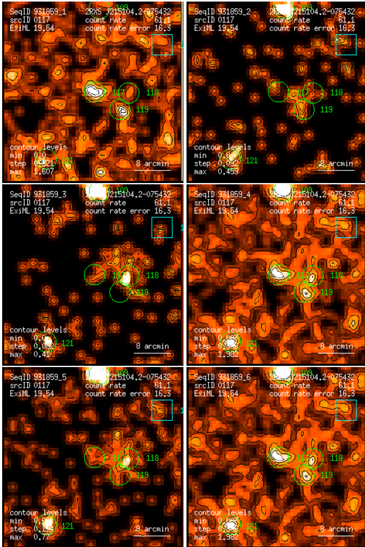
Figure 117: RASS 931859: detection 0117: band rate images, Gaussian filter: (1) PSPC channels 11 – 41, (2) 52 – 90, (3) 91 – 201, (4) 11 – 235, (5) 52 – 201, (6) 11 – 201. Broad band rates in counts/ks. Band rate contour levels in counts/ks/arcmin 2 .
