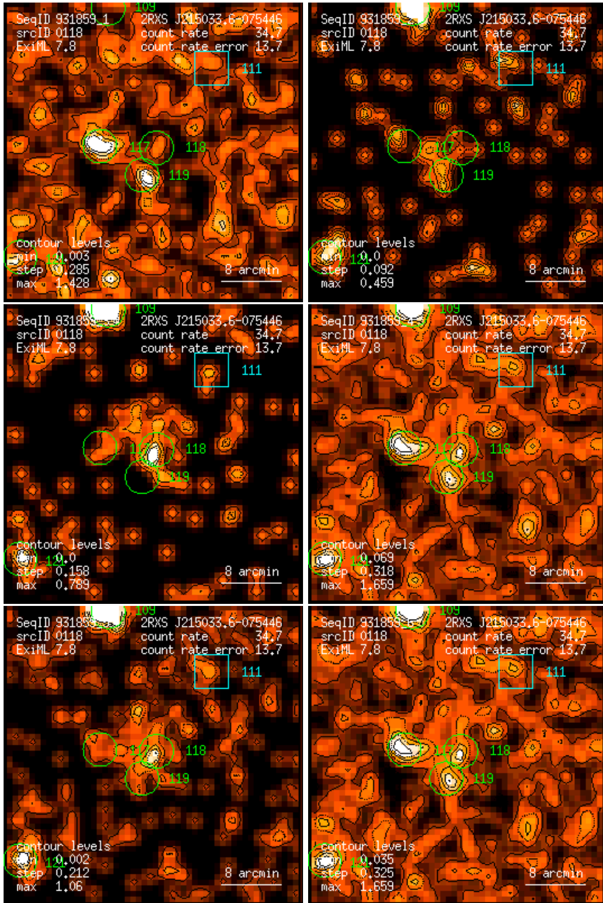
Figure 118: RASS 931859: detection 0118: band rate images, Gaussian filter: (1) PSPC channels 11 – 41, (2) 52 – 90, (3) 91 – 201, (4) 11 – 235, (5) 52 – 201, (6) 11 – 201. Broad band rates in counts/ks. Band rate contour levels in counts/ks/arcmin 2 .
