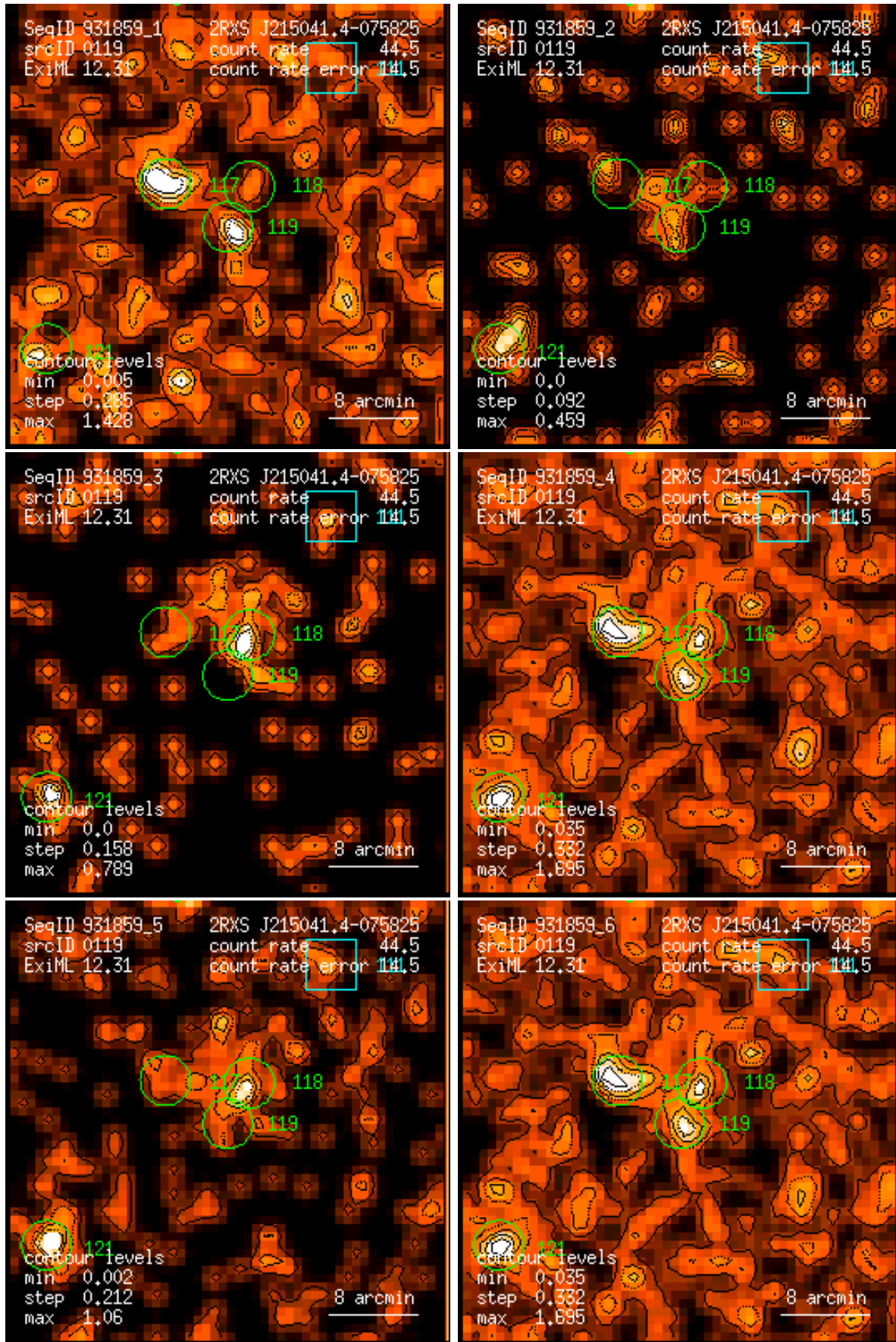
Figure 119: RASS 931859: detection 0119: band rate images, Gaussian filter: (1) PSPC channels 11 – 41, (2) 52 – 90, (3) 91 – 201, (4) 11 – 235, (5) 52 – 201, (6) 11 – 201. Broad band rates in counts/ks. Band rate contour levels in counts/ks/arcmin 2 .
