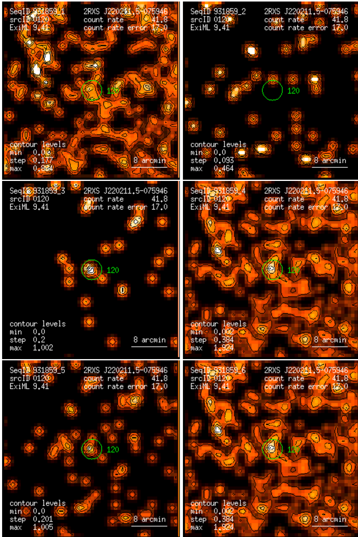
Figure 120: RASS 931859: detection 0120: band rate images, Gaussian filter: (1) PSPC channels 11 – 41, (2) 52 – 90, (3) 91 – 201, (4) 11 – 235, (5) 52 – 201, (6) 11 – 201. Broad band rates in counts/ks. Band rate contour levels in counts/ks/arcmin 2 .
