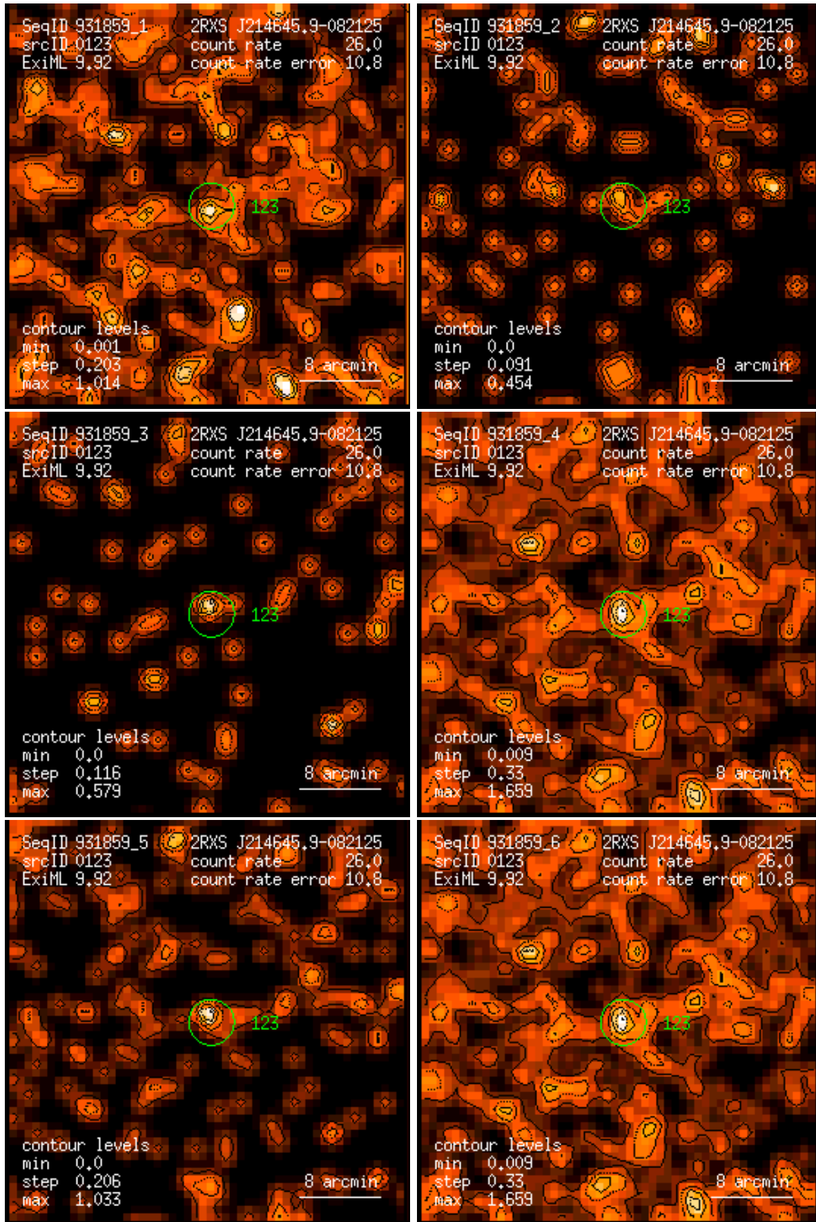
Figure 123: RASS 931859: detection 0123: band rate images, Gaussian filter: (1) PSPC channels 11 – 41, (2) 52 – 90, (3) 91 – 201, (4) 11 – 235, (5) 52 – 201, (6) 11 – 201. Broad band rates in counts/ks. Band rate contour levels in counts/ks/arcmin 2 .
