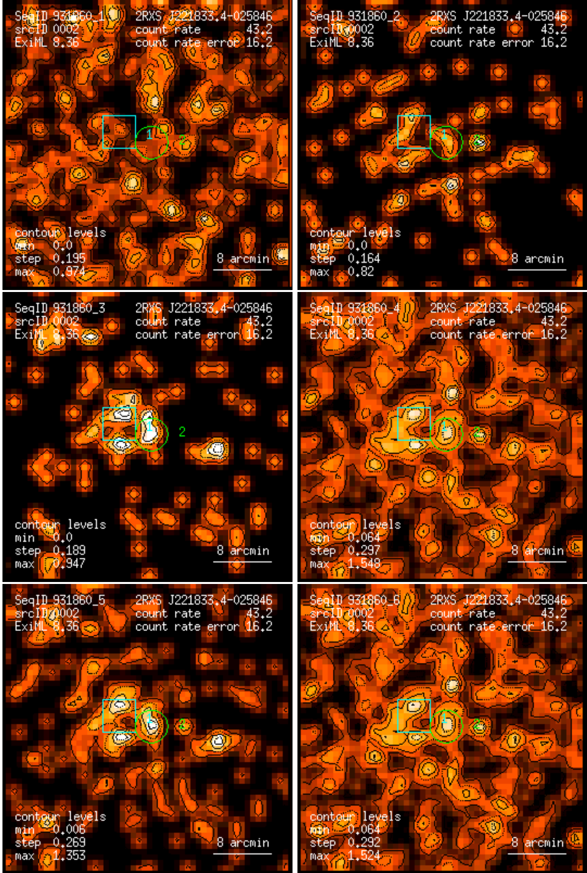
Figure 2: RASS 931860: detection 0002: band rate images, Gaussian filter: (1) PSPC channels 11 – 41, (2) 52 – 90, (3) 91 – 201, (4) 11 – 235, (5) 52 – 201, (6) 11 – 201. Broad band rates in counts/ks. Band rate contour levels in counts/ks/arcmin 2 .
