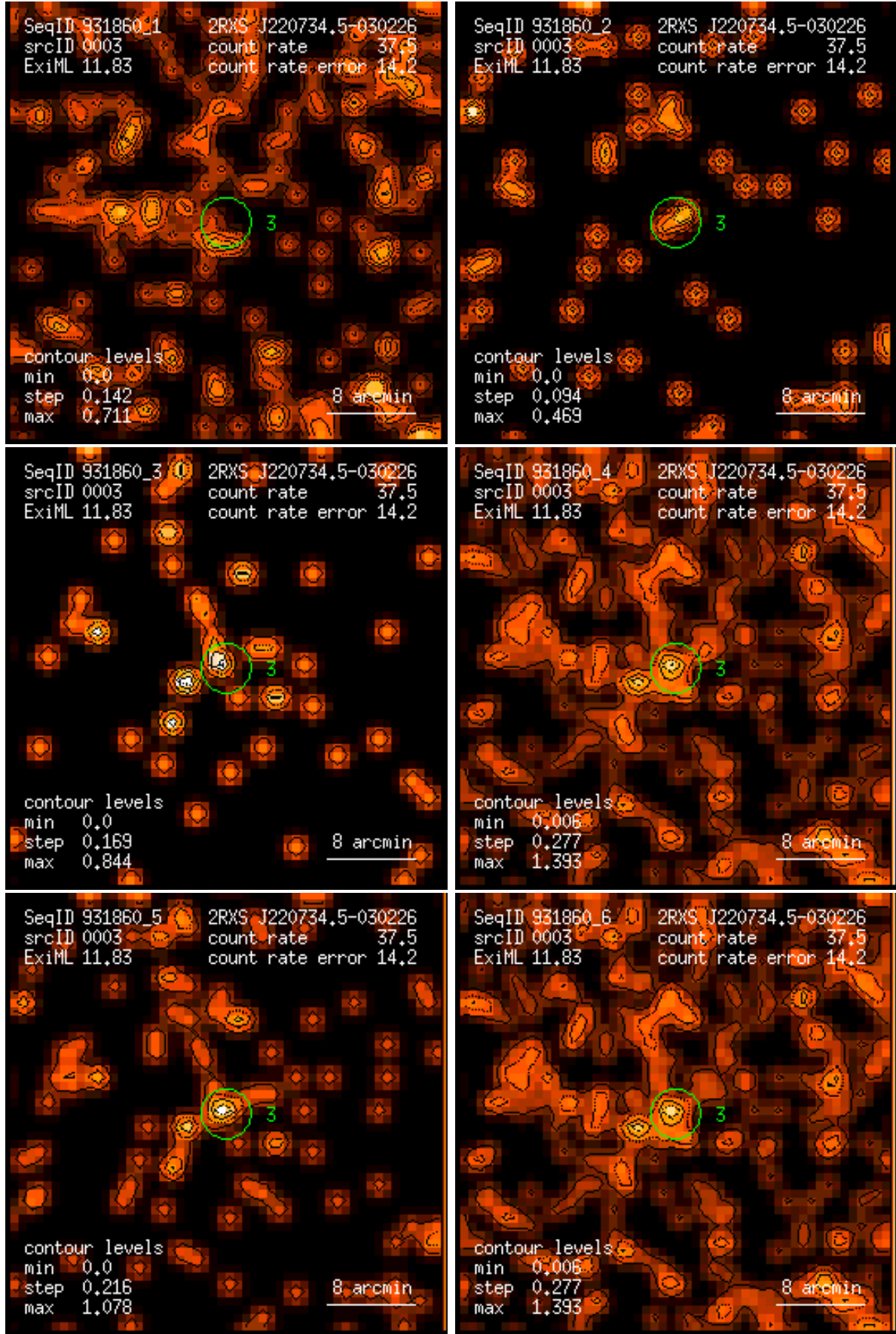
Figure 3: RASS 931860: detection 0003: band rate images, Gaussian filter: (1) PSPC channels 11 – 41, (2) 52 – 90, (3) 91 – 201, (4) 11 – 235, (5) 52 – 201, (6) 11 – 201. Broad band rates in counts/ks. Band rate contour levels in counts/ks/arcmin 2 .
