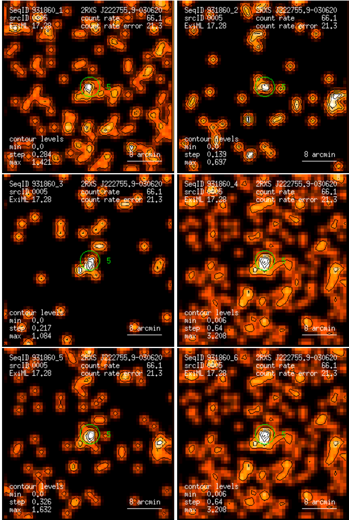
Figure 5: RASS 931860: detection 0005: band rate images, Gaussian filter: (1) PSPC channels 11 – 41, (2) 52 – 90, (3) 91 – 201, (4) 11 – 235, (5) 52 – 201, (6) 11 – 201. Broad band rates in counts/ks. Band rate contour levels in counts/ks/arcmin 2 .
