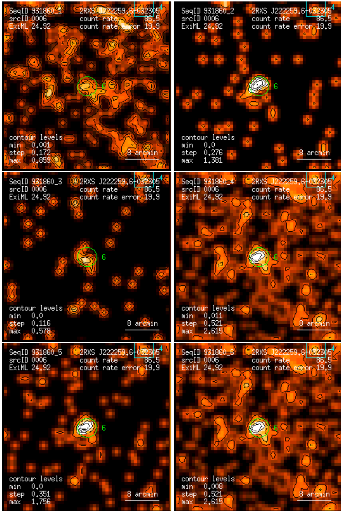
Figure 6: RASS 931860: detection 0006: band rate images, Gaussian filter: (1) PSPC channels 11 – 41, (2) 52 – 90, (3) 91 – 201, (4) 11 – 235, (5) 52 – 201, (6) 11 – 201. Broad band rates in counts/ks. Band rate contour levels in counts/ks/arcmin 2 .
