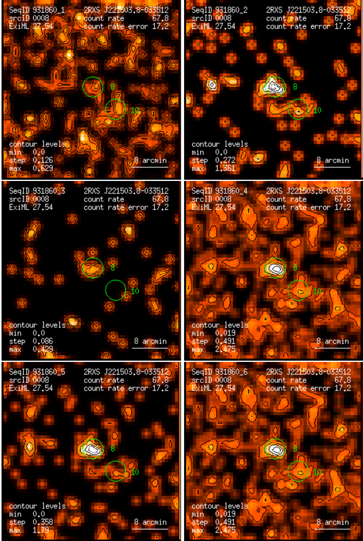
Figure 8: RASS 931860: detection 0008: band rate images, Gaussian filter: (1) PSPC channels 11 – 41, (2) 52 – 90, (3) 91 – 201, (4) 11 – 235, (5) 52 – 201, (6) 11 – 201. Broad band rates in counts/ks. Band rate contour levels in counts/ks/arcmin 2 .
