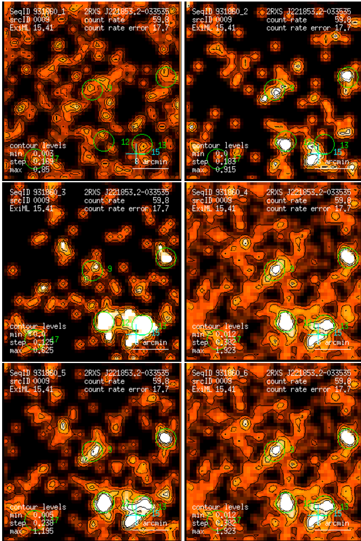
Figure 9: RASS 931860: detection 0009: band rate images, Gaussian filter: (1) PSPC channels 11 – 41, (2) 52 – 90, (3) 91 – 201, (4) 11 – 235, (5) 52 – 201, (6) 11 – 201. Broad band rates in counts/ks. Band rate contour levels in counts/ks/arcmin 2 .
