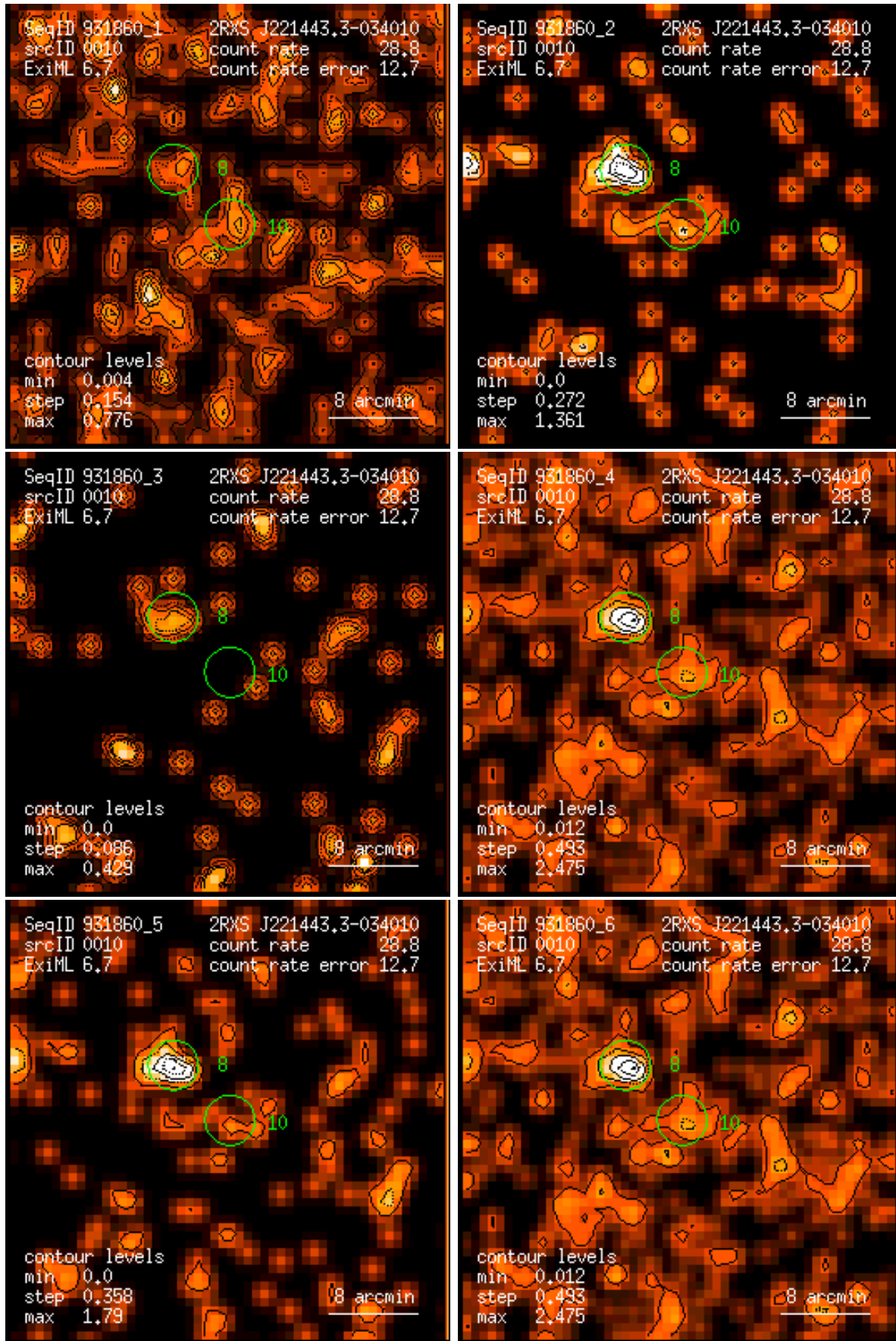
Figure 10: RASS 931860: detection 0010: band rate images, Gaussian filter: (1) PSPC channels 11 – 41, (2) 52 – 90, (3) 91 – 201, (4) 11 – 235, (5) 52 – 201, (6) 11 – 201. Broad band rates in counts/ks. Band rate contour levels in counts/ks/arcmin 2 .
