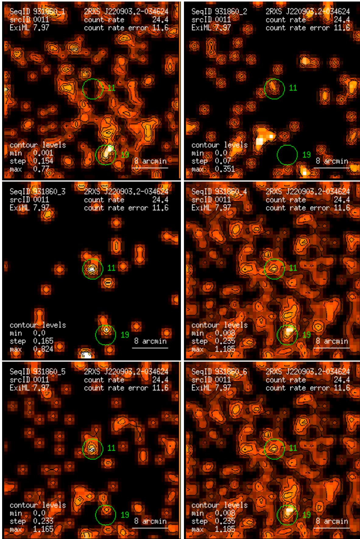
Figure 11: RASS 931860: detection 0011: band rate images, Gaussian filter: (1) PSPC channels 11 – 41, (2) 52 – 90, (3) 91 – 201, (4) 11 – 235, (5) 52 – 201, (6) 11 – 201. Broad band rates in counts/ks. Band rate contour levels in counts/ks/arcmin 2 .
