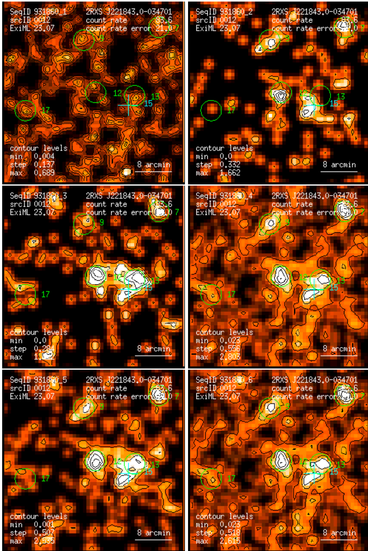
Figure 12: RASS 931860: detection 0012: band rate images, Gaussian filter: (1) PSPC channels 11 – 41, (2) 52 – 90, (3) 91 – 201, (4) 11 – 235, (5) 52 – 201, (6) 11 – 201. Broad band rates in counts/ks. Band rate contour levels in counts/ks/arcmin 2 .
