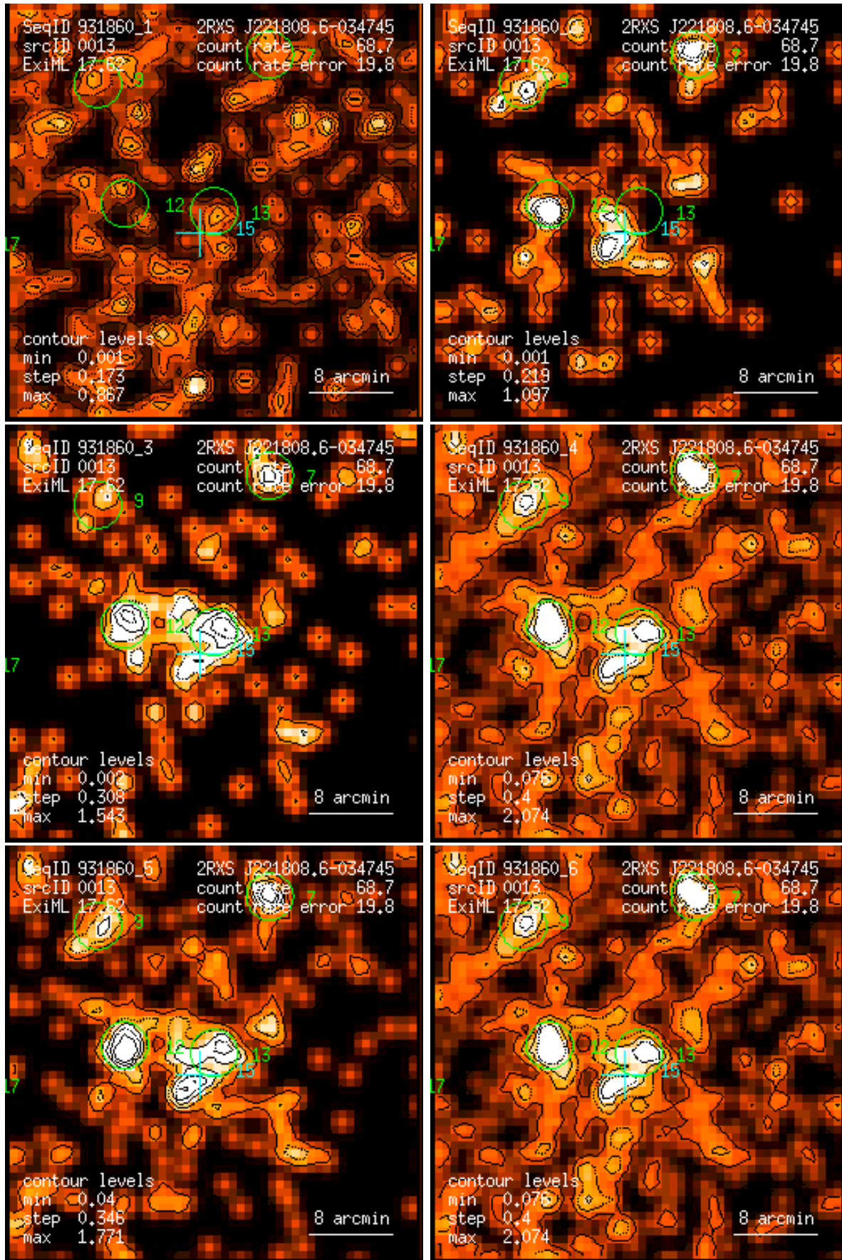
Figure 13: RASS 931860: detection 0013: band rate images, Gaussian filter: (1) PSPC channels 11 – 41, (2) 52 – 90, (3) 91 – 201, (4) 11 – 235, (5) 52 – 201, (6) 11 – 201. Broad band rates in counts/ks. Band rate contour levels in counts/ks/arcmin 2 .
