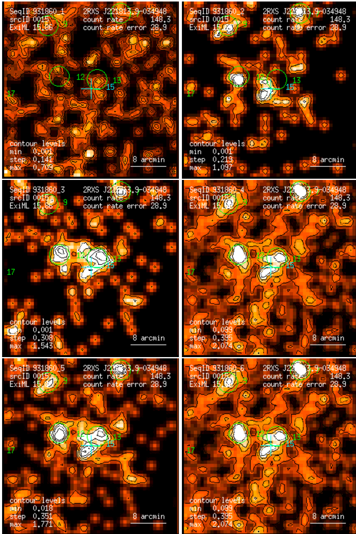
Figure 15: RASS 931860: detection 0015: band rate images, Gaussian filter: (1) PSPC channels 11 – 41, (2) 52 – 90, (3) 91 – 201, (4) 11 – 235, (5) 52 – 201, (6) 11 – 201. Broad band rates in counts/ks. Band rate contour levels in counts/ks/arcmin 2 .
