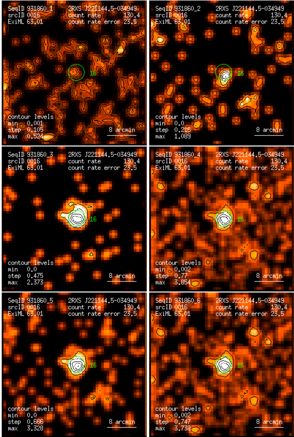
Figure 16: RASS 931860: detection 0016: band rate images, Gaussian filter: (1) PSPC channels 11 – 41, (2) 52 – 90, (3) 91 – 201, (4) 11 – 235, (5) 52 – 201, (6) 11 – 201. Broad band rates in counts/ks. Band rate contour levels in counts/ks/arcmin 2 .
