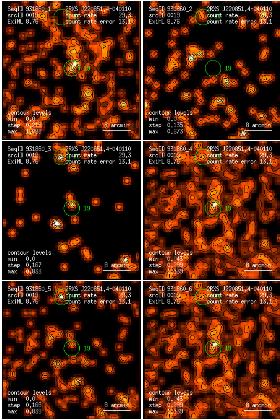
Figure 19: RASS 931860: detection 0019: band rate images, Gaussian filter: (1) PSPC channels 11 – 41, (2) 52 – 90, (3) 91 – 201, (4) 11 – 235, (5) 52 – 201, (6) 11 – 201. Broad band rates in counts/ks. Band rate contour levels in counts/ks/arcmin 2 .
