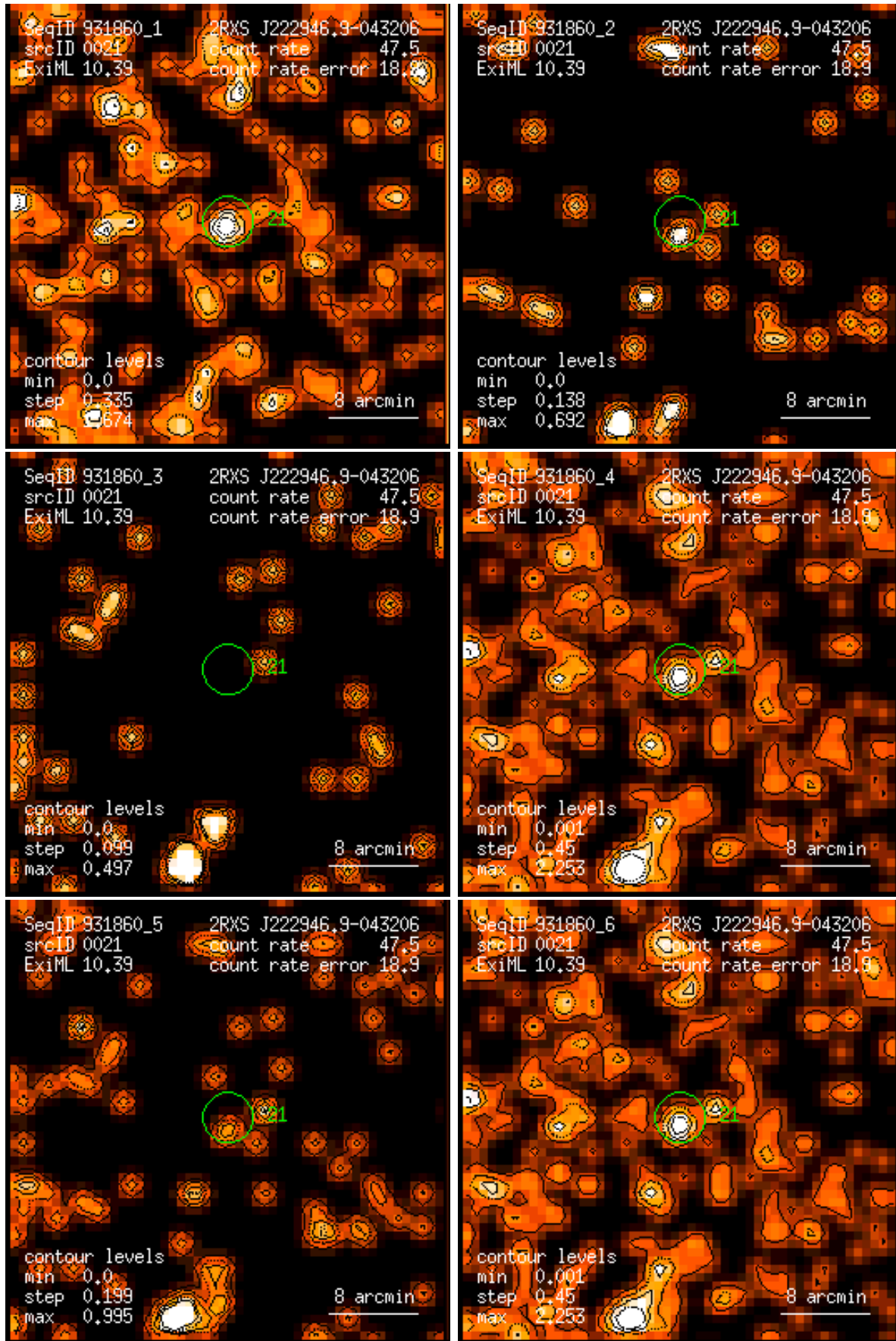
Figure 21: RASS 931860: detection 0021: band rate images, Gaussian filter: (1) PSPC channels 11 – 41, (2) 52 – 90, (3) 91 – 201, (4) 11 – 235, (5) 52 – 201, (6) 11 – 201. Broad band rates in counts/ks. Band rate contour levels in counts/ks/arcmin 2 .
