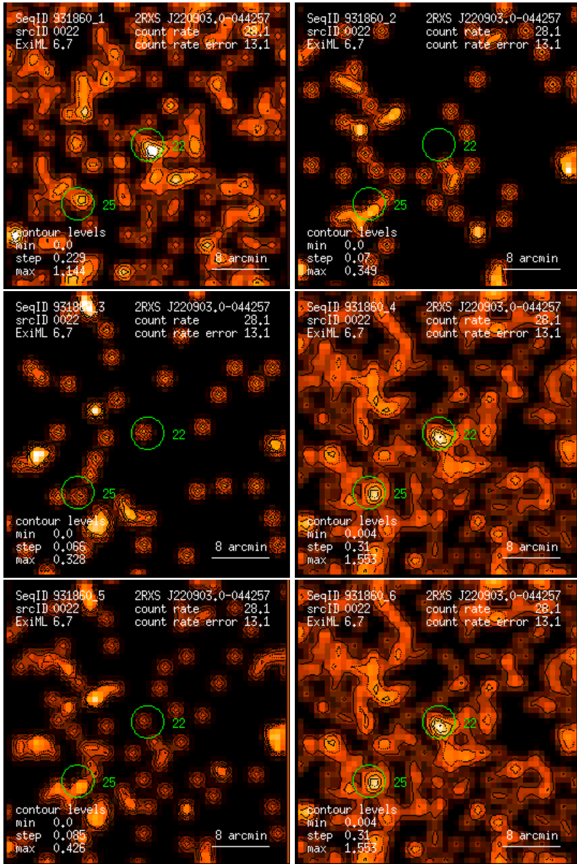
Figure 22: RASS 931860: detection 0022: band rate images, Gaussian filter: (1) PSPC channels 11 – 41, (2) 52 – 90, (3) 91 – 201, (4) 11 – 235, (5) 52 – 201, (6) 11 – 201. Broad band rates in counts/ks. Band rate contour levels in counts/ks/arcmin 2 .
