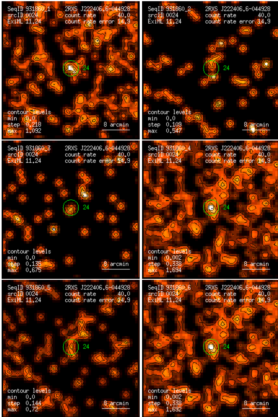
Figure 24: RASS 931860: detection 0024: band rate images, Gaussian filter: (1) PSPC channels 11 – 41, (2) 52 – 90, (3) 91 – 201, (4) 11 – 235, (5) 52 – 201, (6) 11 – 201. Broad band rates in counts/ks. Band rate contour levels in counts/ks/arcmin 2 .
