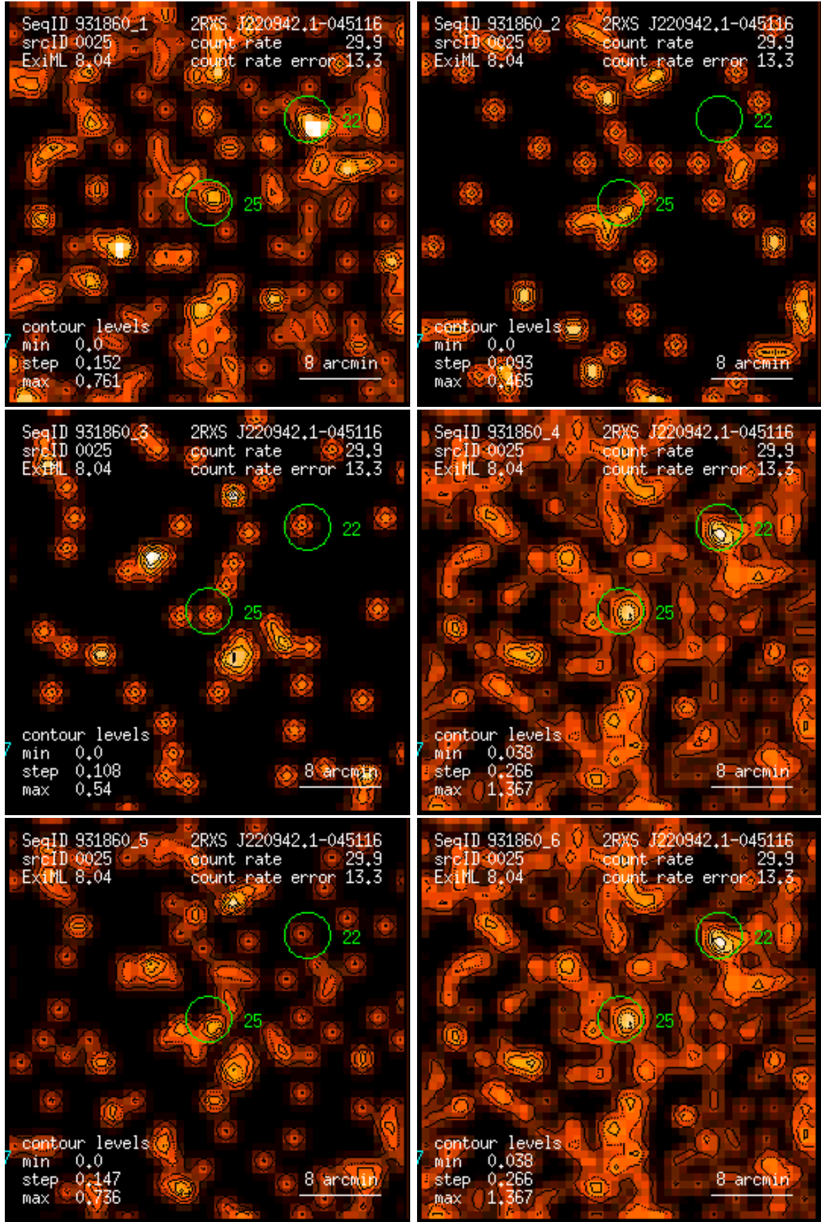
Figure 25: RASS 931860: detection 0025: band rate images, Gaussian filter: (1) PSPC channels 11 – 41, (2) 52 – 90, (3) 91 – 201, (4) 11 – 235, (5) 52 – 201, (6) 11 – 201. Broad band rates in counts/ks. Band rate contour levels in counts/ks/arcmin 2 .
