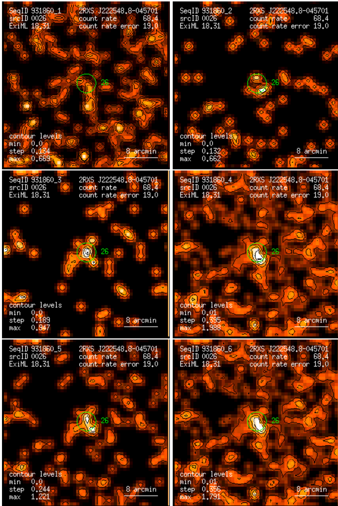
Figure 26: RASS 931860: detection 0026: band rate images, Gaussian filter: (1) PSPC channels 11 – 41, (2) 52 – 90, (3) 91 – 201, (4) 11 – 235, (5) 52 – 201, (6) 11 – 201. Broad band rates in counts/ks. Band rate contour levels in counts/ks/arcmin 2 .
