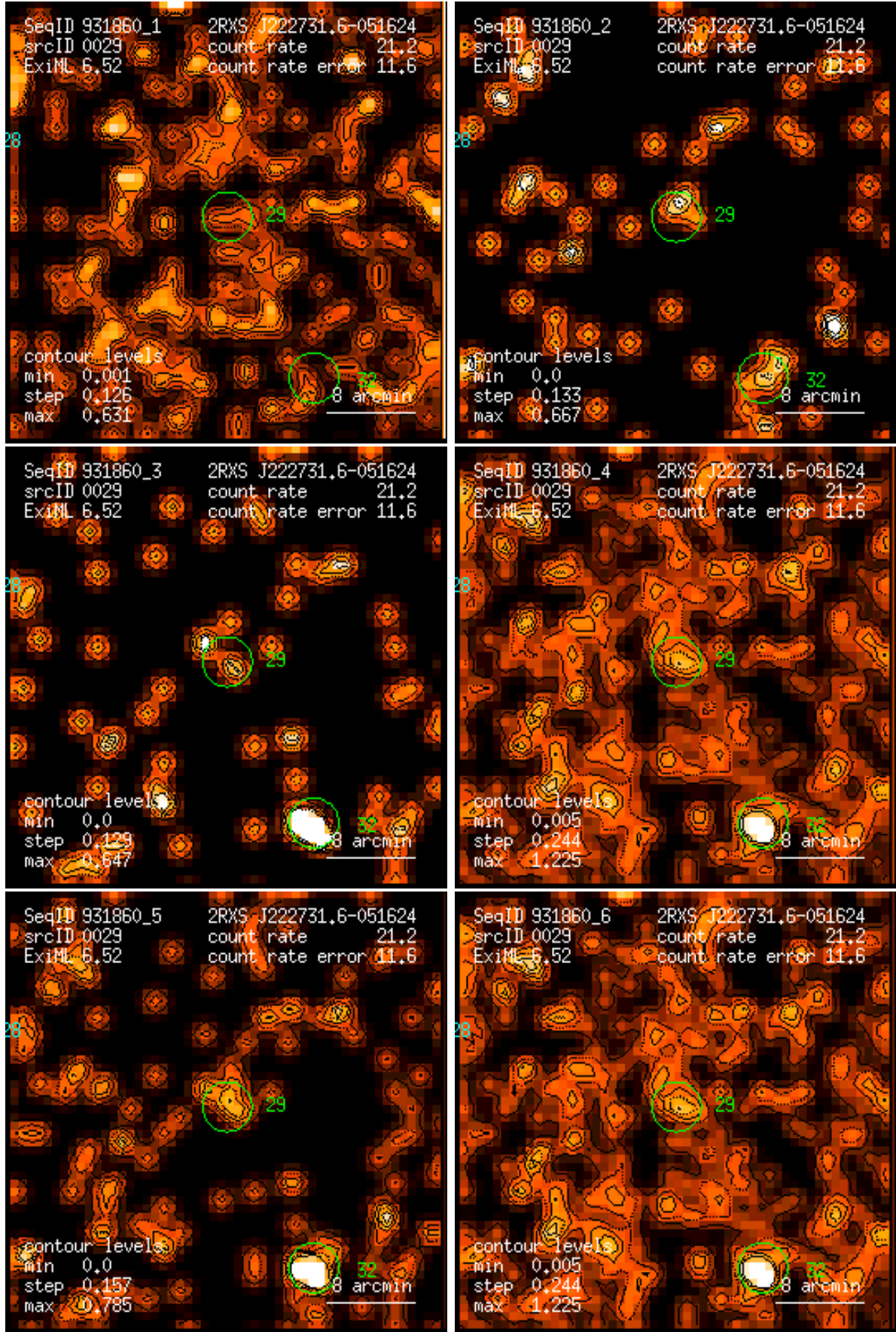
Figure 29: RASS 931860: detection 0029: band rate images, Gaussian filter: (1) PSPC channels 11 – 41, (2) 52 – 90, (3) 91 – 201, (4) 11 – 235, (5) 52 – 201, (6) 11 – 201. Broad band rates in counts/ks. Band rate contour levels in counts/ks/arcmin 2 .
