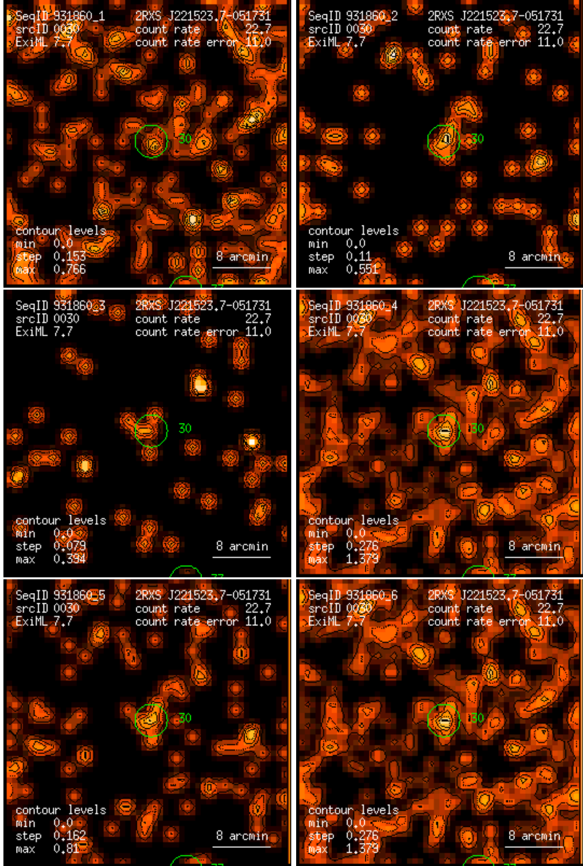
Figure 30: RASS 931860: detection 0030: band rate images, Gaussian filter: (1) PSPC channels 11 – 41, (2) 52 – 90, (3) 91 – 201, (4) 11 – 235, (5) 52 – 201, (6) 11 – 201. Broad band rates in counts/ks. Band rate contour levels in counts/ks/arcmin 2 .
