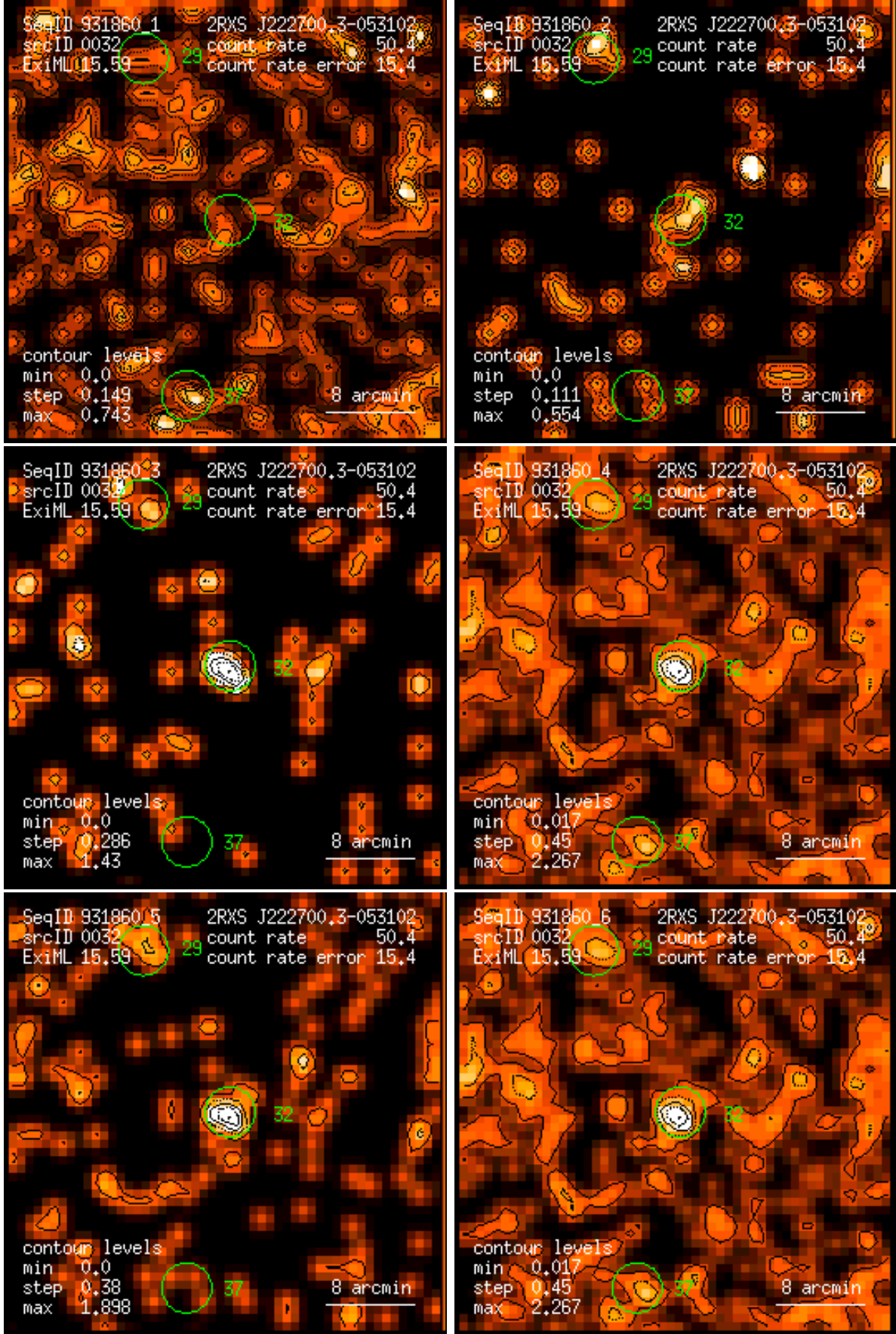
Figure 32: RASS 931860: detection 0032: band rate images, Gaussian filter: (1) PSPC channels 11 – 41, (2) 52 – 90, (3) 91 – 201, (4) 11 – 235, (5) 52 – 201, (6) 11 – 201. Broad band rates in counts/ks. Band rate contour levels in counts/ks/arcmin 2 .
