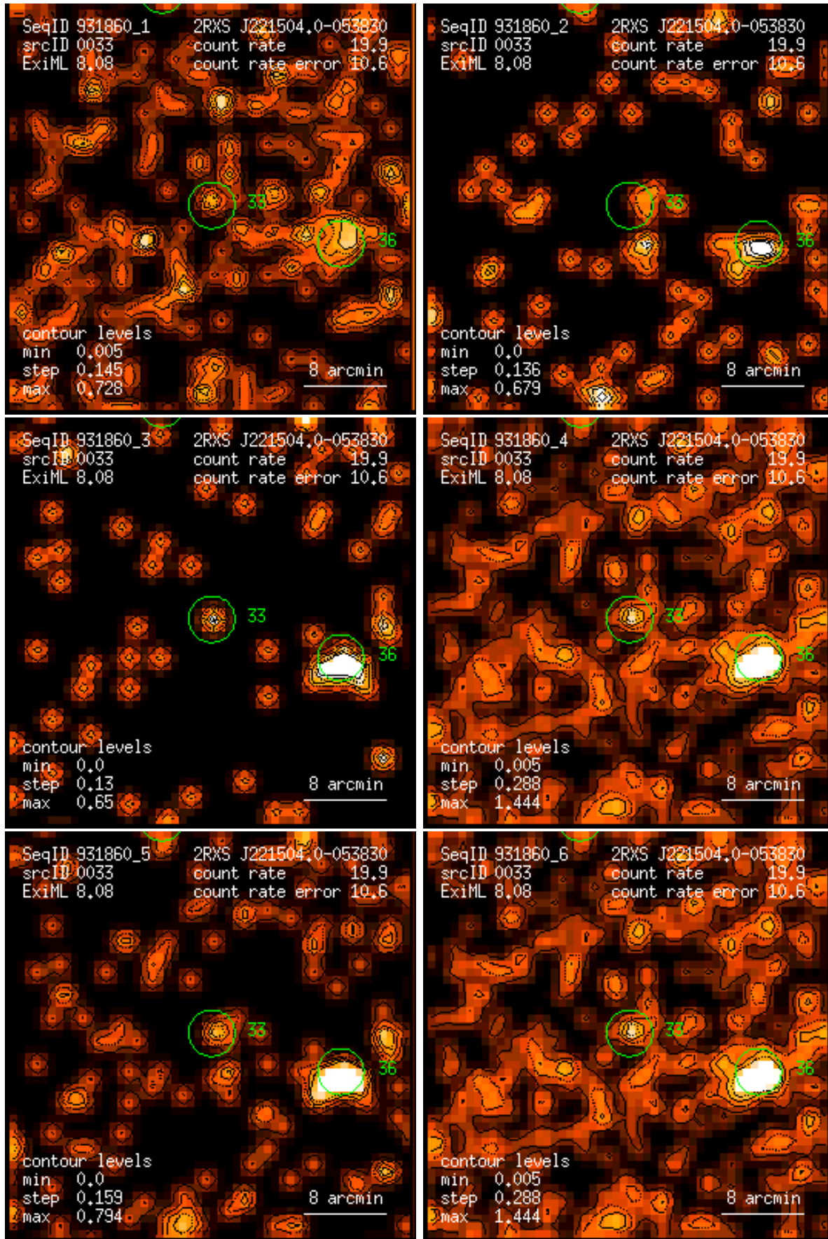
Figure 33: RASS 931860: detection 0033: band rate images, Gaussian filter: (1) PSPC channels 11 – 41, (2) 52 – 90, (3) 91 – 201, (4) 11 – 235, (5) 52 – 201, (6) 11 – 201. Broad band rates in counts/ks. Band rate contour levels in counts/ks/arcmin 2 .
