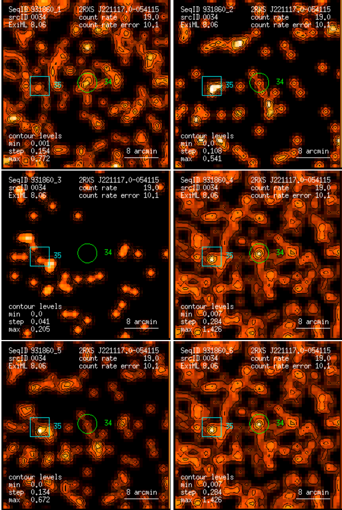
Figure 34: RASS 931860: detection 0034: band rate images, Gaussian filter: (1) PSPC channels 11 – 41, (2) 52 – 90, (3) 91 – 201, (4) 11 – 235, (5) 52 – 201, (6) 11 – 201. Broad band rates in counts/ks. Band rate contour levels in counts/ks/arcmin 2 .
