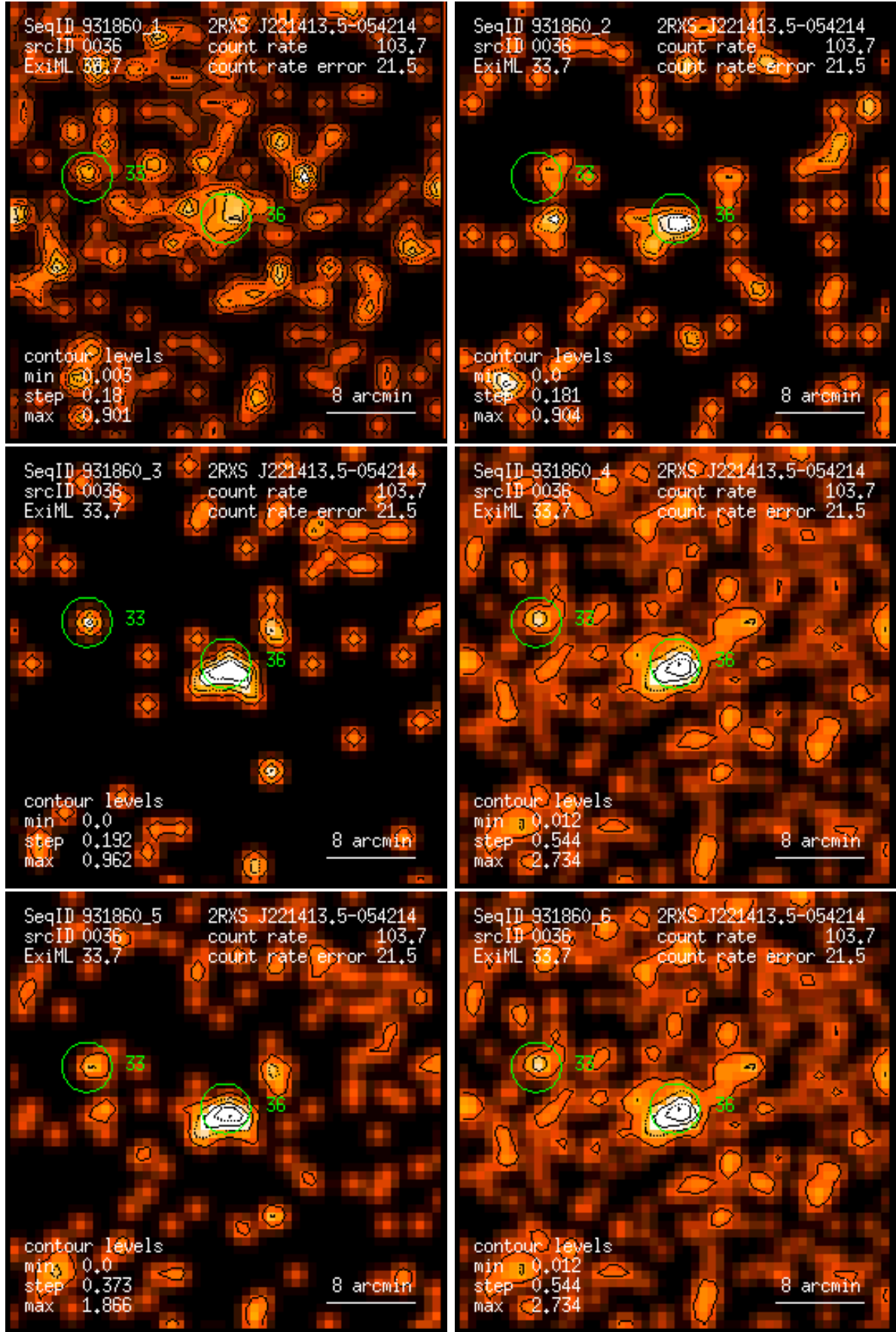
Figure 36: RASS 931860: detection 0036: band rate images, Gaussian filter: (1) PSPC channels 11 – 41, (2) 52 – 90, (3) 91 – 201, (4) 11 – 235, (5) 52 – 201, (6) 11 – 201. Broad band rates in counts/ks. Band rate contour levels in counts/ks/arcmin 2 .
