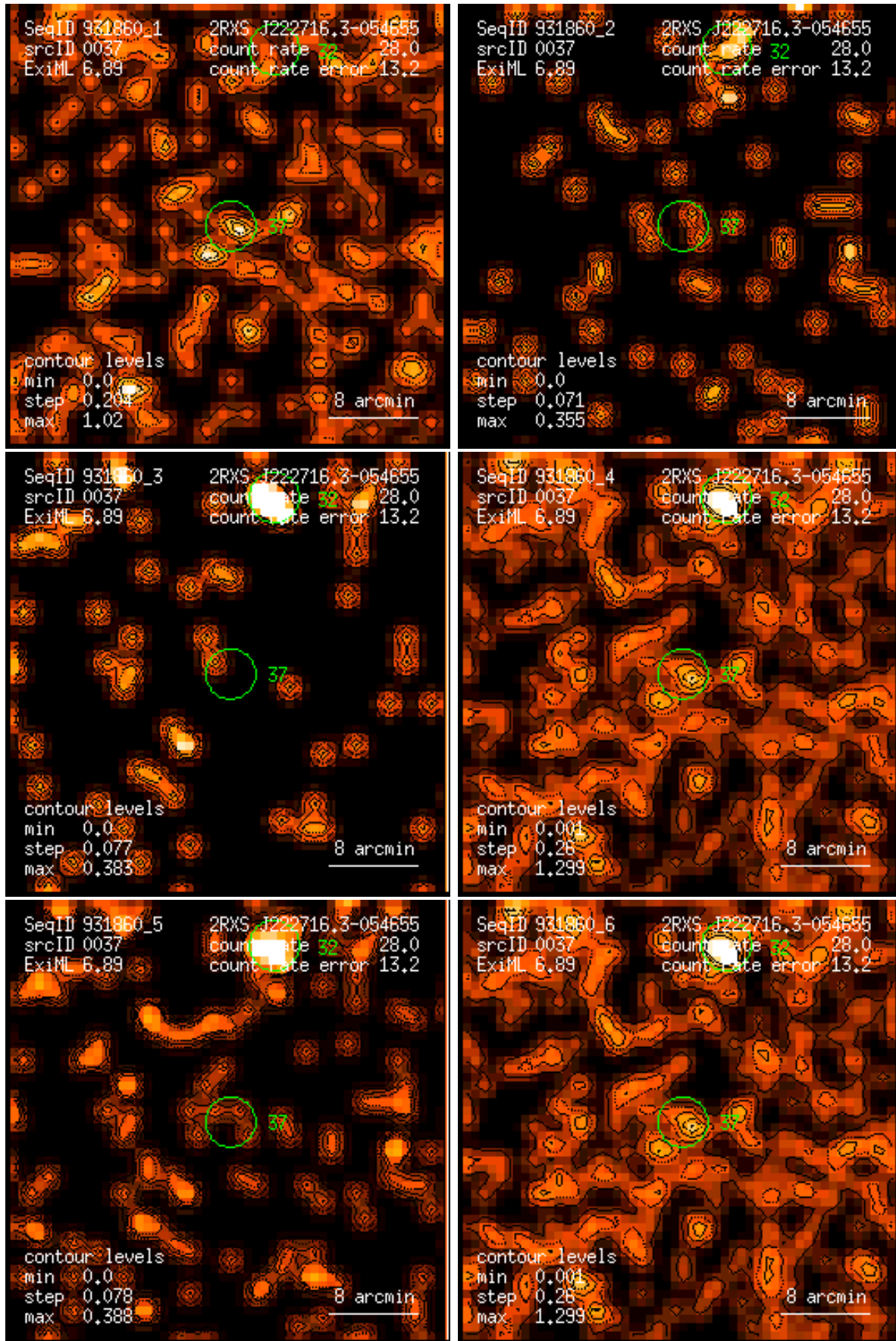
Figure 37: RASS 931860: detection 0037: band rate images, Gaussian filter: (1) PSPC channels 11 – 41, (2) 52 – 90, (3) 91 – 201, (4) 11 – 235, (5) 52 – 201, (6) 11 – 201. Broad band rates in counts/ks. Band rate contour levels in counts/ks/arcmin 2 .
