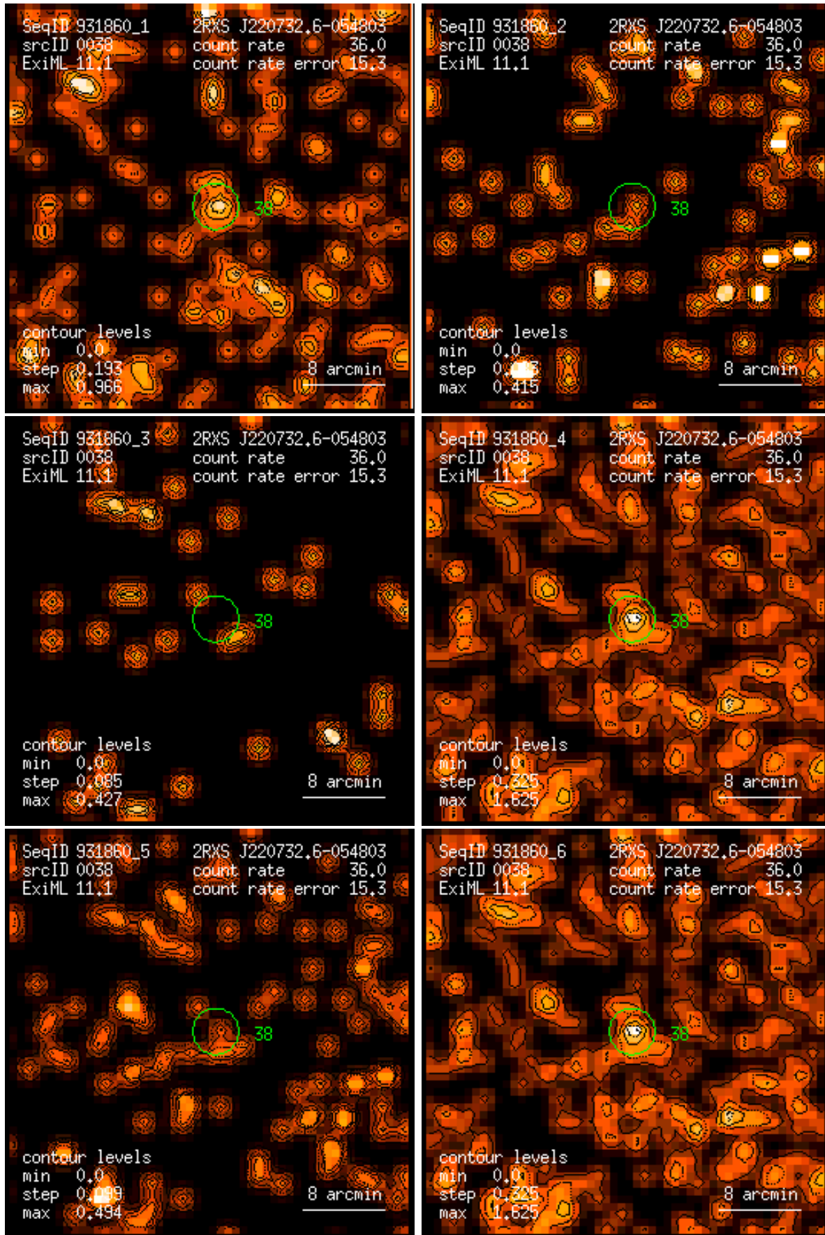
Figure 38: RASS 931860: detection 0038: band rate images, Gaussian filter: (1) PSPC channels 11 – 41, (2) 52 – 90, (3) 91 – 201, (4) 11 – 235, (5) 52 – 201, (6) 11 – 201. Broad band rates in counts/ks. Band rate contour levels in counts/ks/arcmin 2 .
