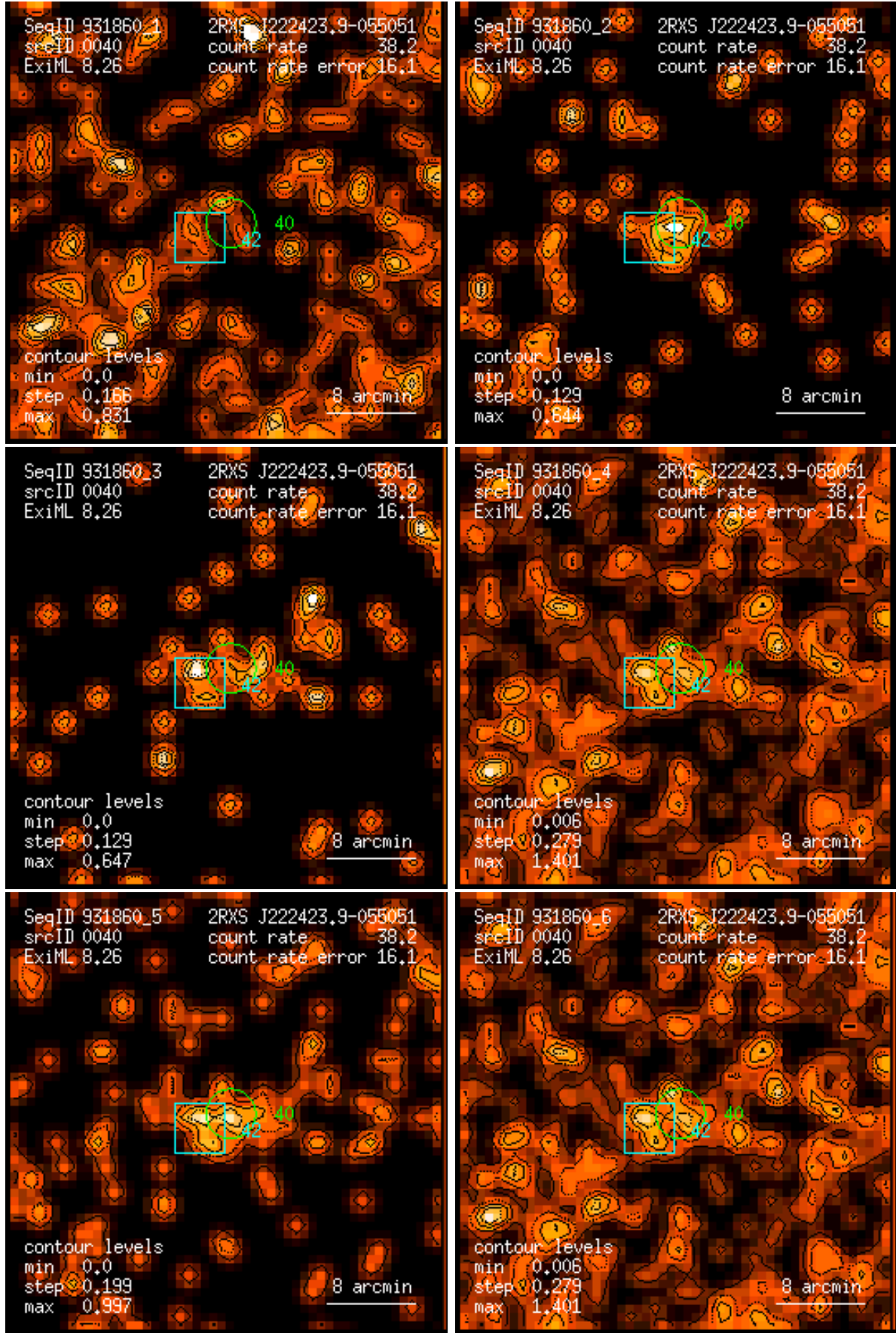
Figure 40: RASS 931860: detection 0040: band rate images, Gaussian filter: (1) PSPC channels 11 – 41, (2) 52 – 90, (3) 91 – 201, (4) 11 – 235, (5) 52 – 201, (6) 11 – 201. Broad band rates in counts/ks. Band rate contour levels in counts/ks/arcmin 2 .
