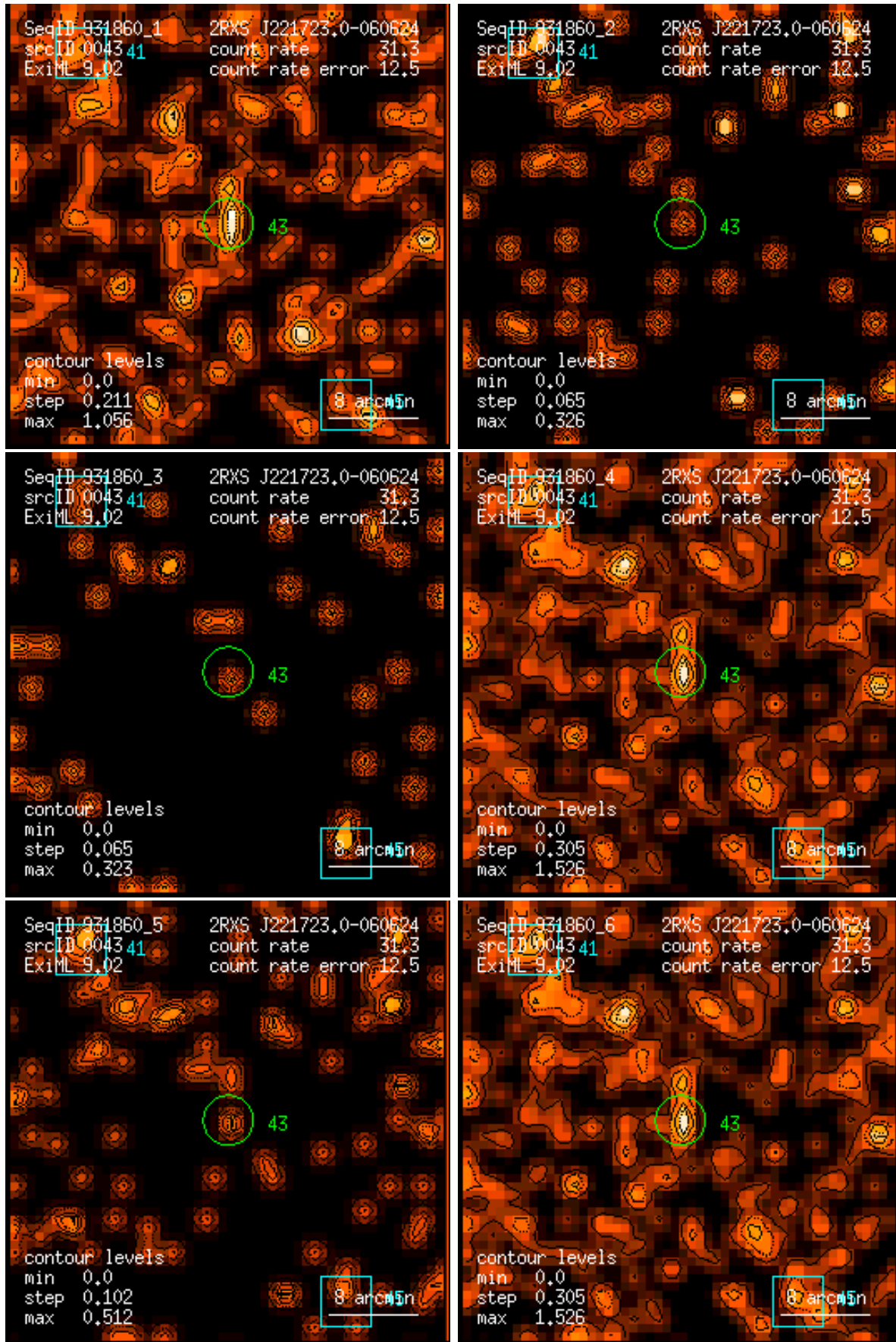
Figure 43: RASS 931860: detection 0043: band rate images, Gaussian filter: (1) PSPC channels 11 – 41, (2) 52 – 90, (3) 91 – 201, (4) 11 – 235, (5) 52 – 201, (6) 11 – 201. Broad band rates in counts/ks. Band rate contour levels in counts/ks/arcmin 2 .
