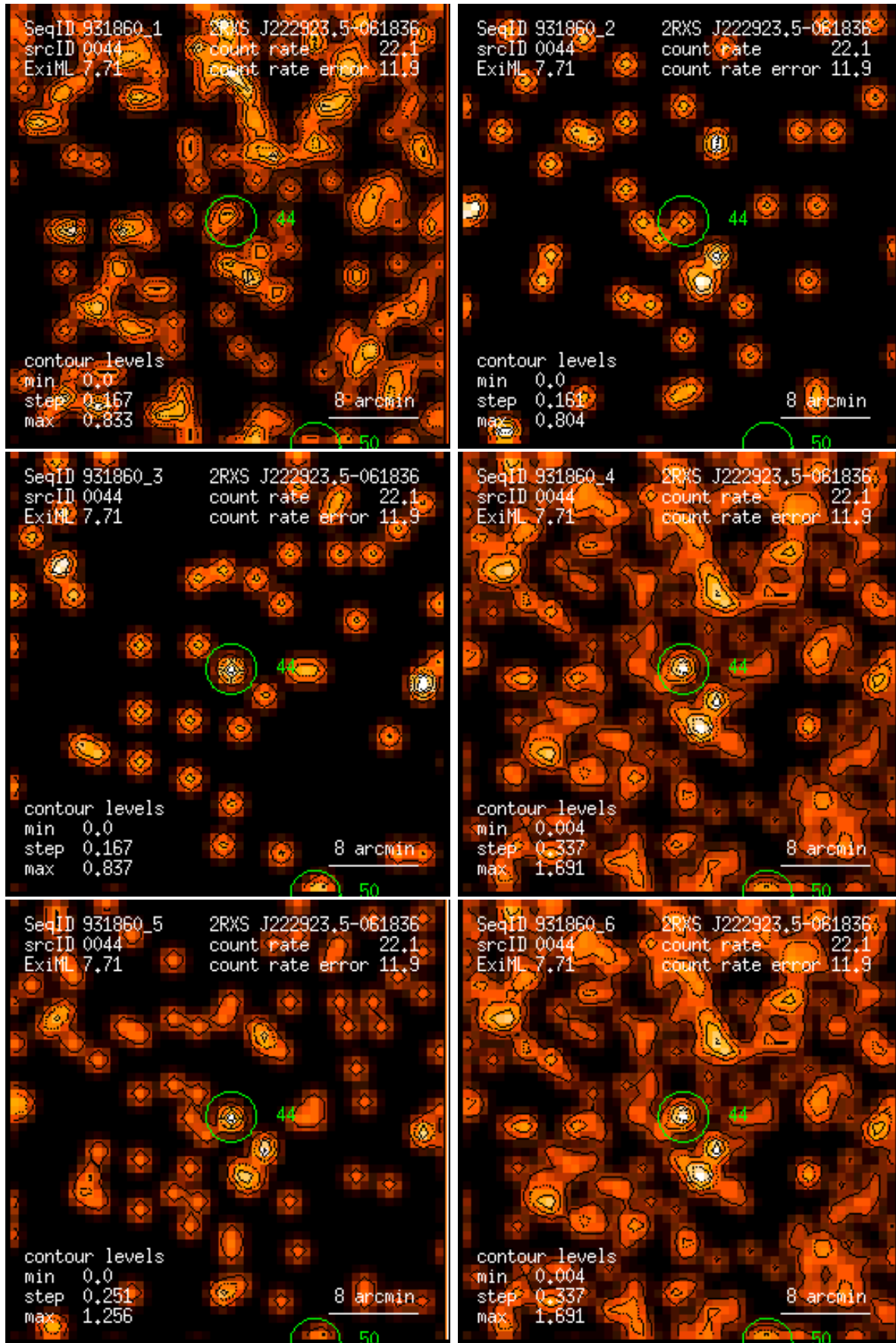
Figure 44: RASS 931860: detection 0044: band rate images, Gaussian filter: (1) PSPC channels 11 – 41, (2) 52 – 90, (3) 91 – 201, (4) 11 – 235, (5) 52 – 201, (6) 11 – 201. Broad band rates in counts/ks. Band rate contour levels in counts/ks/arcmin 2 .
