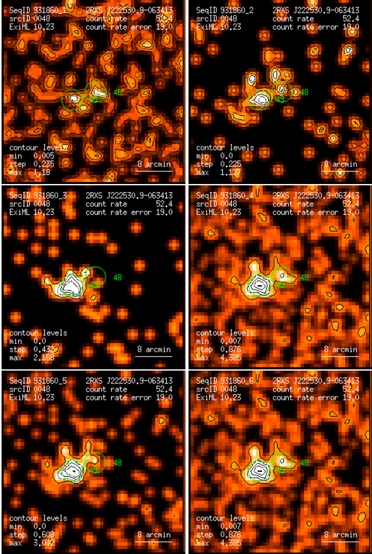
Figure 48: RASS 931860: detection 0048: band rate images, Gaussian filter: (1) PSPC channels 11 – 41, (2) 52 – 90, (3) 91 – 201, (4) 11 – 235, (5) 52 – 201, (6) 11 – 201. Broad band rates in counts/ks. Band rate contour levels in counts/ks/arcmin 2 .
