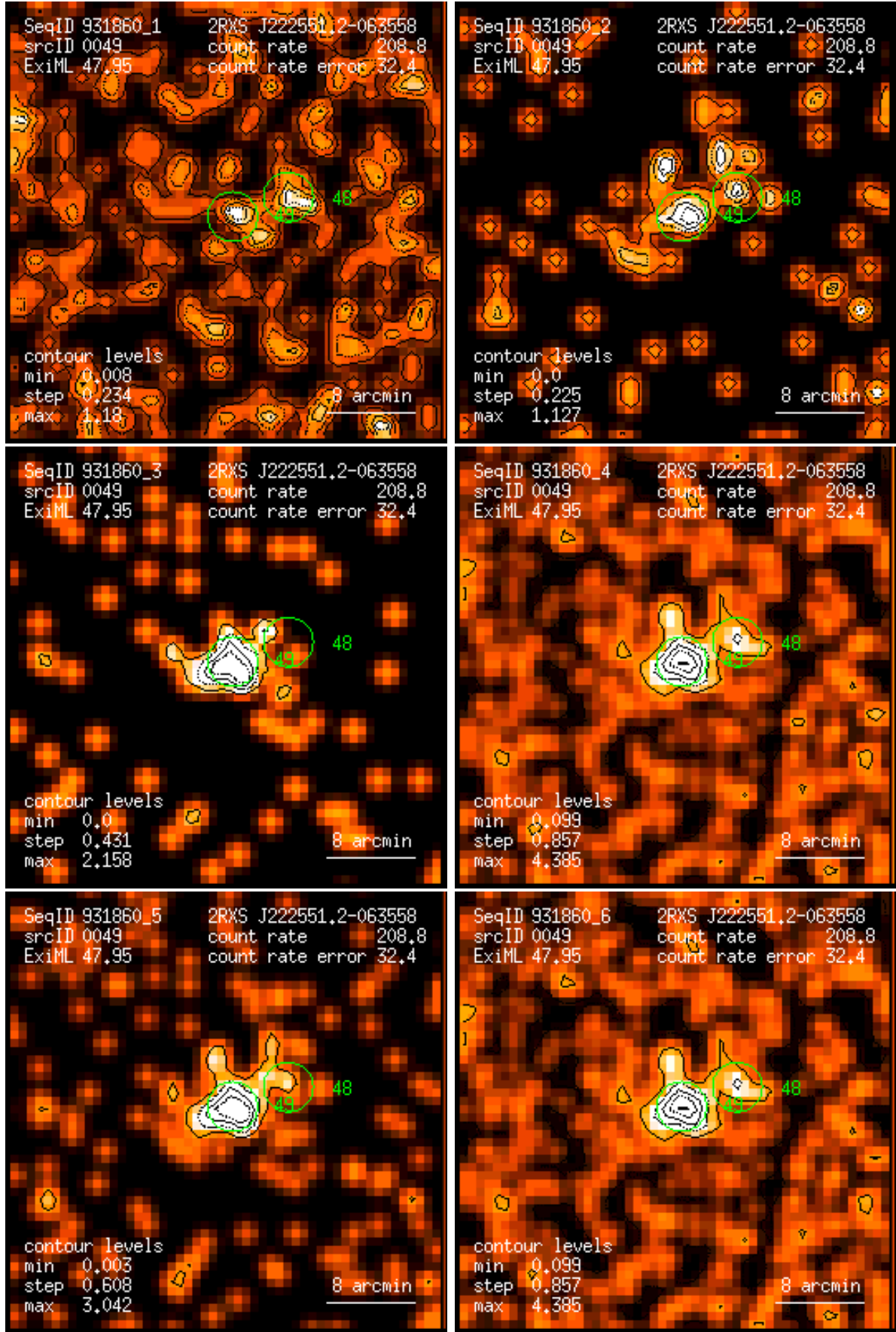
Figure 49: RASS 931860: detection 0049: band rate images, Gaussian filter: (1) PSPC channels 11 – 41, (2) 52 – 90, (3) 91 – 201, (4) 11 – 235, (5) 52 – 201, (6) 11 – 201. Broad band rates in counts/ks. Band rate contour levels in counts/ks/arcmin 2 .
