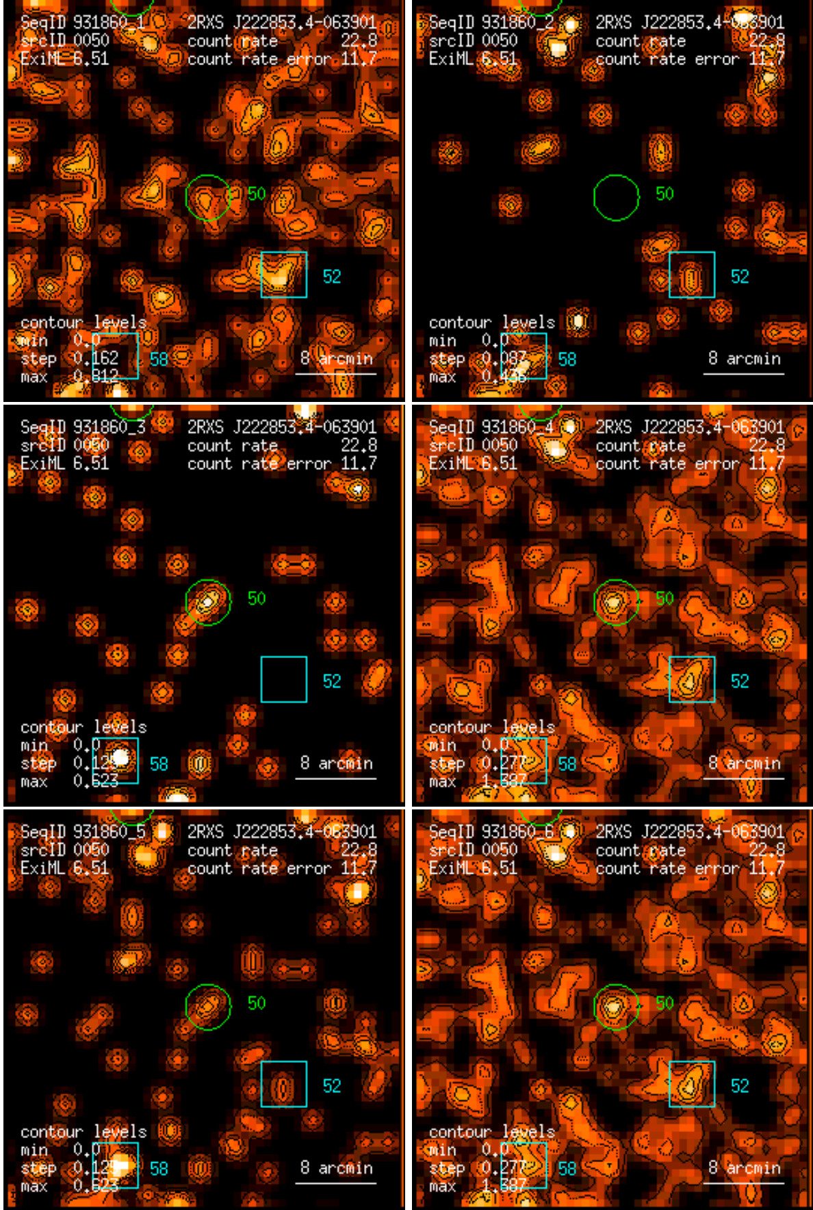
Figure 50: RASS 931860: detection 0050: band rate images, Gaussian filter: (1) PSPC channels 11 – 41, (2) 52 – 90, (3) 91 – 201, (4) 11 – 235, (5) 52 – 201, (6) 11 – 201. Broad band rates in counts/ks. Band rate contour levels in counts/ks/arcmin 2 .
